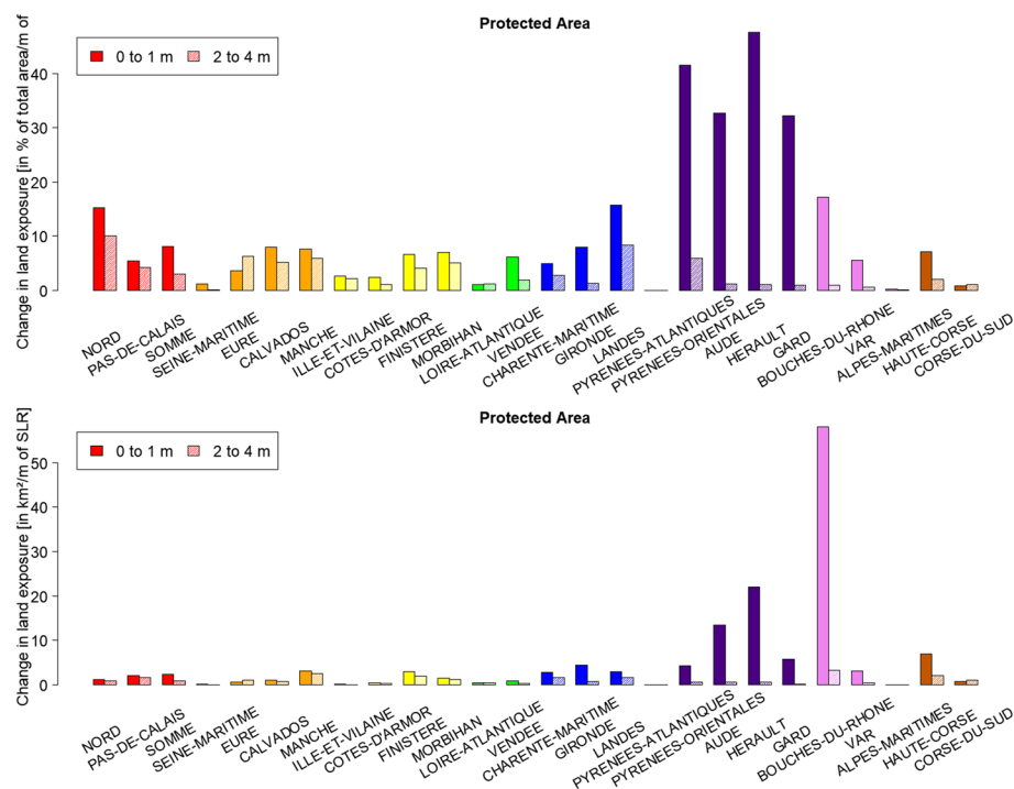
Fig. 6 Rate of change in Cdl low-lying land exposure with respect to SLR. Rates are shown in relative (in % of total land area/m of SLR) and absolute (in \text{km}^2/\text{m} of SLR) values on the top and bottom panel, respectively. For each NUTS3 regions, rates are calculated for the SLR ranges 0–1 m (filled bars, left) and 2–4 m (hatched bars, right)
