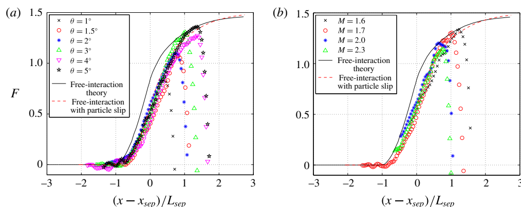
FIGURE 20. (Colour online) Correlation function F for a range of flow deflection angles (a) and free stream Mach numbers (b).
