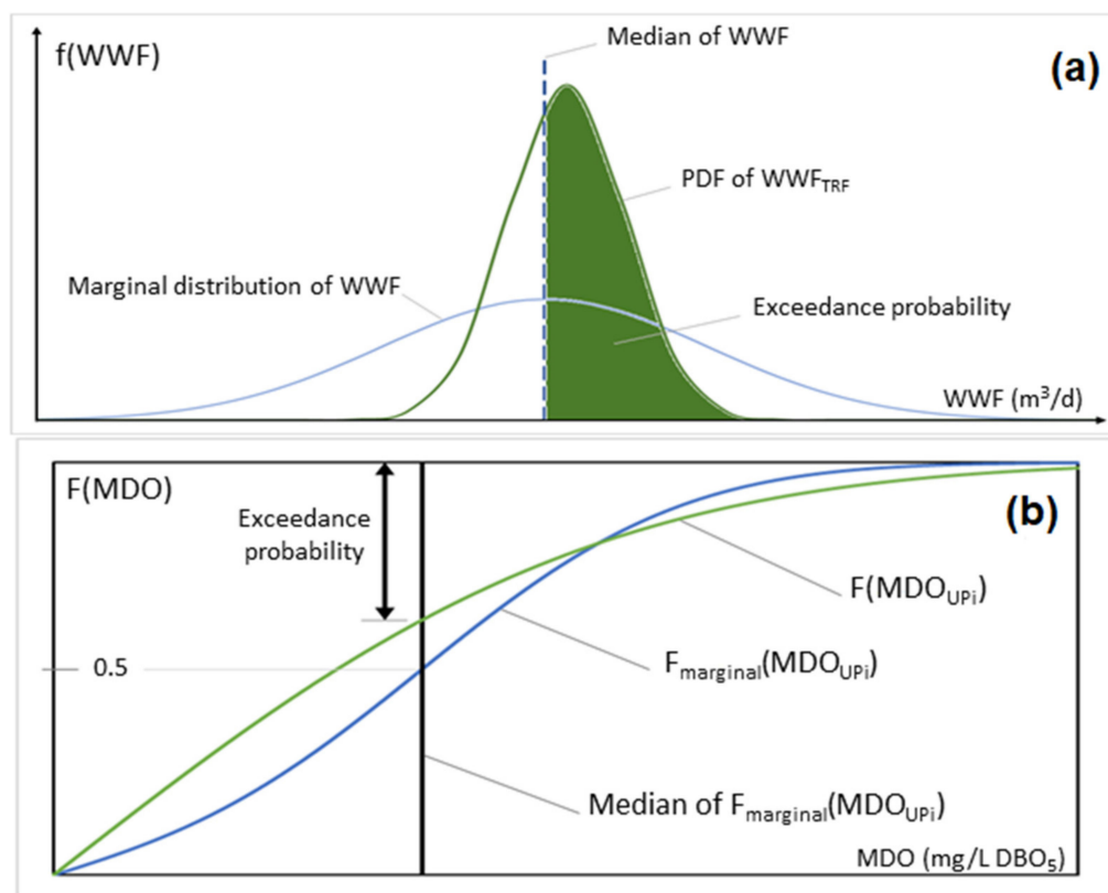
Figure 4. Conditional probabilities determination by (a) PDF and by (b) cumulative PDF.
