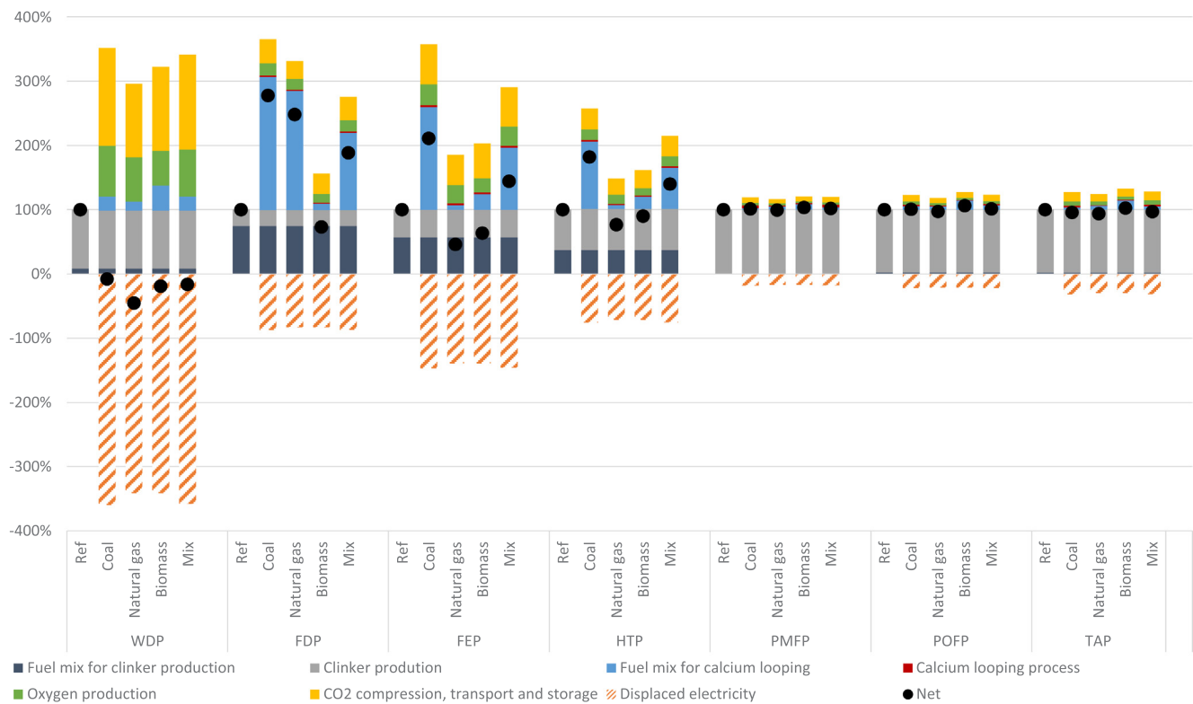
Fig. 5. Results of the calcium looping cases relative to the reference case without CO 2 capture for the other environmental impacts categories: water depletion potential (WDP), fossil depletion potential (FDP), freshwater eutrophication potential (FEP), human toxicity potential (HTP), particulate matter formation (PMF), photochemical oxidant formation (POF), and terrestrial acidification potential (TAP).
