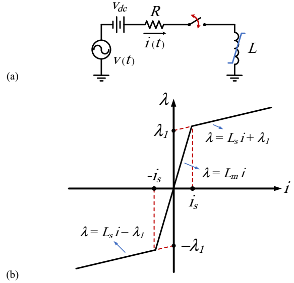
Fig. 1. The basis for mathematical analysis. (a) Non-linear equivalent circuit under study. (b) The assumed magnetization characteristic.
