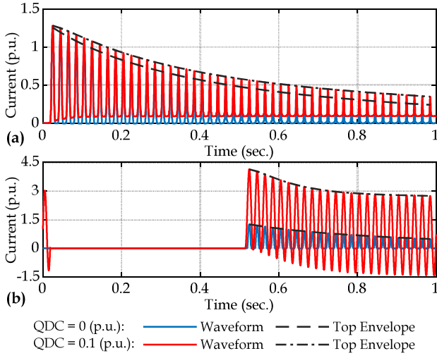
Fig. 2. Inrush current waveforms of the simple circuit under study. (a) Energization inrush currents. (b) Recovery inrush currents.
