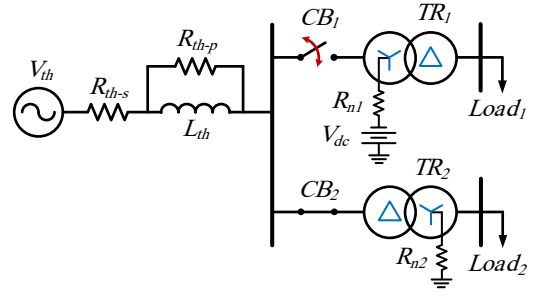
Fig. 3. Simulated system for analyzing QDCs' impact on inrush currents.
