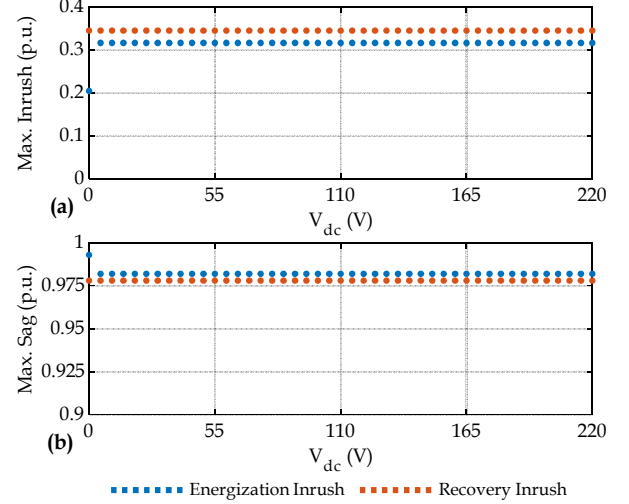
Fig. 10. Effect of proposed mitigation strategy on energization and recovery under QDCs: (a) on maximum drawn currents in the primary of TR_1 , (b) on maximum voltage sag experienced in the secondary of TR_2 .
