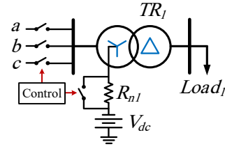
Fig. 9. Proposed scheme based on controlled switching for phase energization and neutral resistance insertion.
