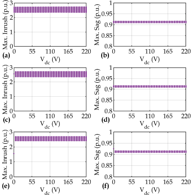
Fig. 5. Effect of ground resistance on energization inrush. Left side: Inrush currents in the primary of TR_1 . Right side: Voltage sags at the secondary of TR_2 . (a) and (b) R_{n1}=2.5\Omega , (c) and (d) R_{n1}=25\Omega , (e) and (f) R_{n1}=250\Omega .
