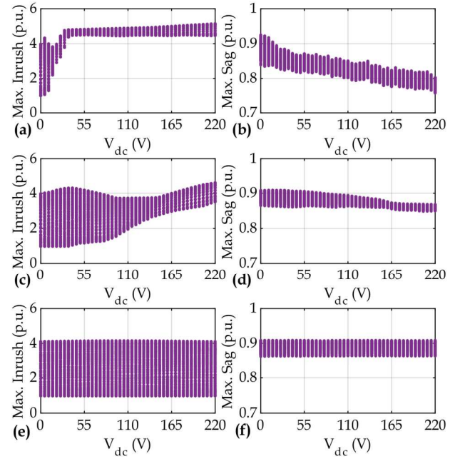
Fig. 6. Effect of ground resistance on recovery inrush. Left side: Inrush currents in the primary of TR_1 . Right side: Voltage sags at the secondary of TR_2 . (a) and (b) R_{n1}=2.5\Omega , (c) and (d) R_{n1}=25\Omega , (e) and (f) R_{n1}=250\Omega .
