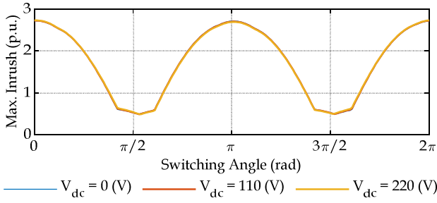
Fig. 7. Effect of switching angle on energization inrush phenomena.
