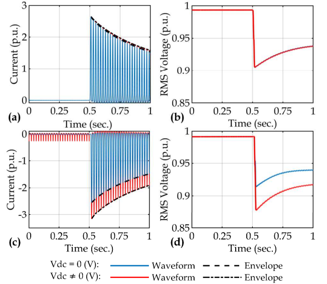
Fig. 4. Impact of QDCs on domestic and sympathetic inrush phenomena during energization and re-energization. (a) Inrush currents in the primary of TR_1 upon energization. (b) Voltage sags at the secondary of TR_2 upon energization. (c) Inrush currents in the primary of TR_1 upon re-energization. (d) Voltage sags at the secondary of TR_2 upon re-energization.
