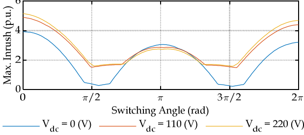
Fig. 8. Effect of switching angle on recovery inrush phenomena. on-wave energization angles of the transformer adversities of inrush currents, even in the presence of QDCs is possible.
