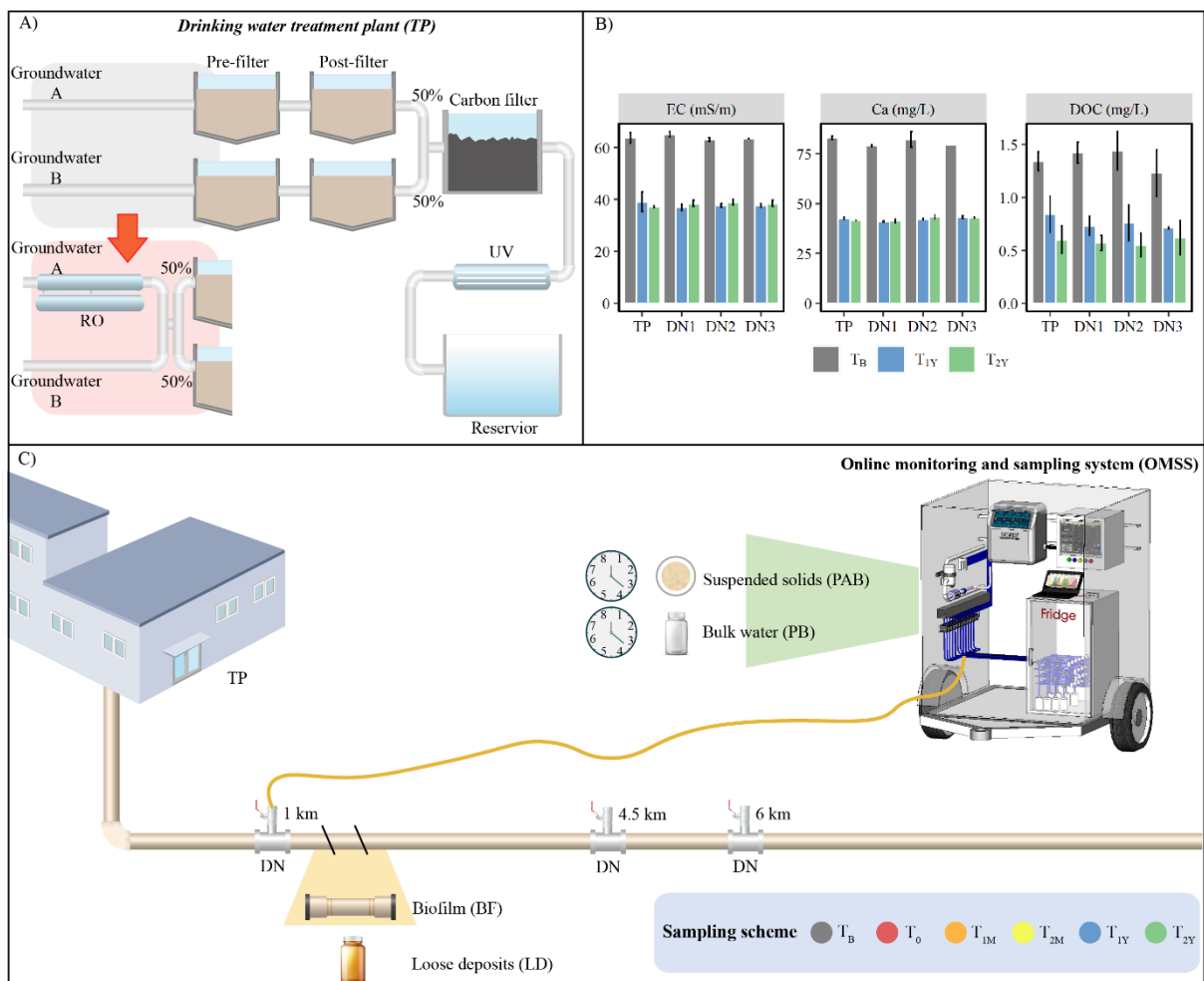
Figure 5-1. A) Water treatment processes before and after introducing RO; B) EC, Ca, and DOC values before ( T_B ), and one year ( T_{1Y} ), 2 years ( T_{2Y} ) after RO introduction at treatment plant (TP) and in distribution network (DN). DN1, DN2 and DN3 stand for locations in
