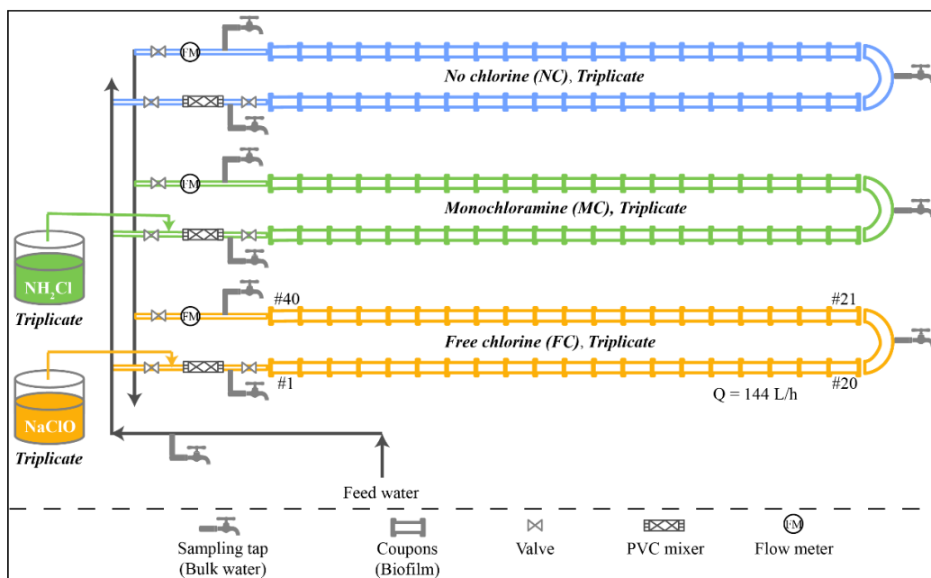
Figure 2-1. The design of the pilot system
