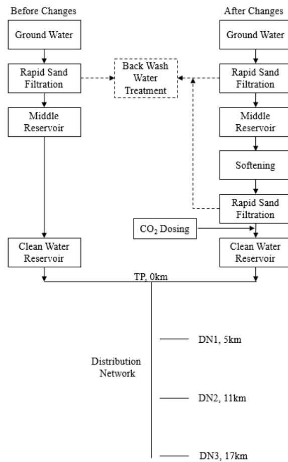
Figure 4-S1. Layout of the treatment processes before and after upgrading. Samples were taken at treatment plant (TP, 0km), DN1 (5km), DN2 (11km) and DN3 (17km).
