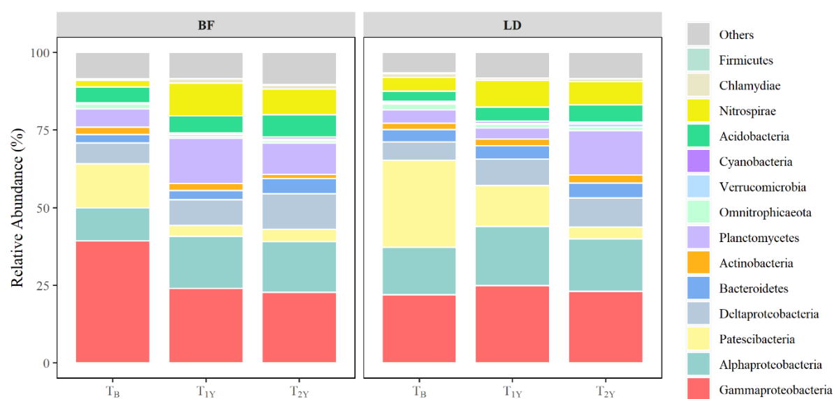
Figure 5-S11. The variations in taxonomy composition at phylum level in distribution network (DN) within biofilm (BF) and loose deposits (LD) over time. T B : before the RO introduction; T 1Y : 1 year after the RO introduction; T 2Y : 2 years after the RO introduction.
