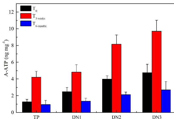
Figure 4-3. Active biomass of suspended particles measured by ATP from treatment plant (TP) to locations in distribution network (DN1, DN2 and DN3) before ( T_0 , black), during ( T_{3\text{-weeks}} , red) and after ( T_{6\text{-months}} , blue) upgrading the treatments. Data are presented as mean \pm s.d. ( n = 3 ).
