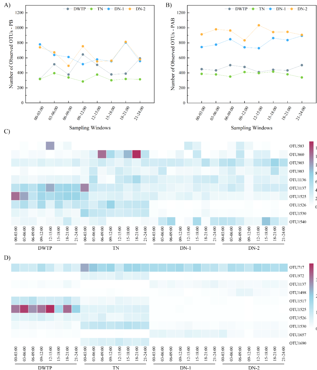
Figure 3-4. The daily variations in the number of observed OTUs and the top 10 dominant OTUs over time and space in DWDS: A) the daily variations in observed OTU numbers for PB; B) the daily variations in observed OTU numbers for PAB; C) the heatmap showing the top 10 dominant OTUs in PB; and D) the heatmap showing the 10 dominant OTUs in PAB. The line plots show the averaged values in the number of observed OTUs from triplicate samples at each time point, while the heatmaps illustrate the averaged relative abundance within each species from triplicate samples at each time point.
