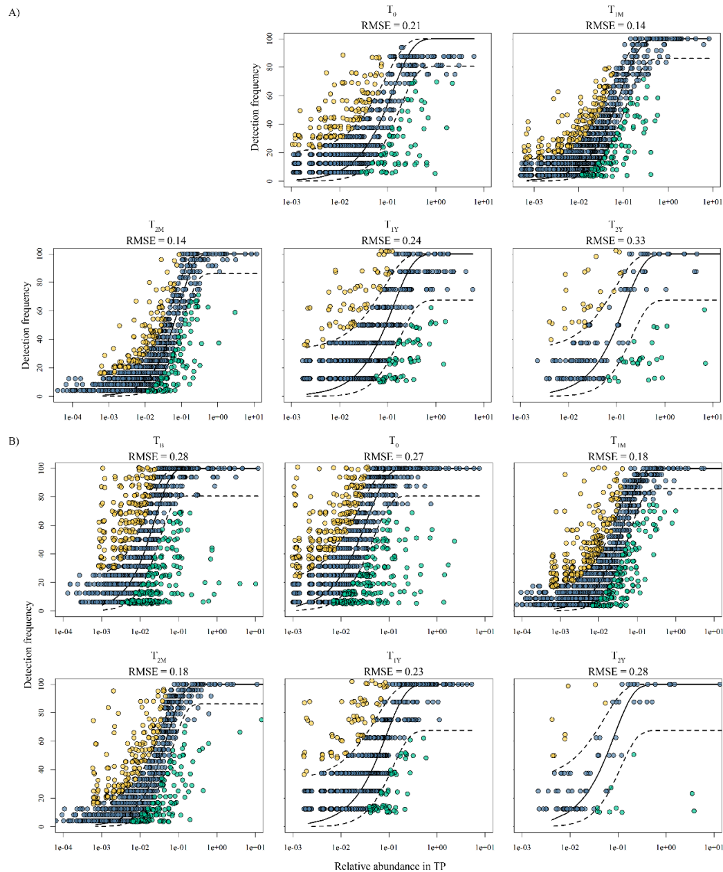
Figure 5-S16. Neutral processes explain microbial community assembly across time. Scatterplot of the prevalence of each ASV in PB (A) and PAB (B) in distribution network (DN) versus its mean relative abundance in PB and PAB at treatment plant (TP) for each time period. The gray line is their predicted distribution (shaded area is 95% confidence interval) based on the neutral community model. Points are colored by the ASV's fit to the model: above prediction – yellow, as prediction – blue, below prediction – green. Average RMSE was calculated from 1000 bootstrap resamplings.
