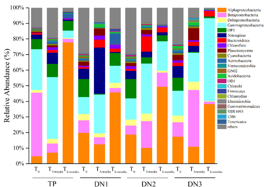
Figure 4-S3. The major phylum (relative abundance > 0.5%) types of bacterial associated with suspended particles at treatment plant and in the distribution system detected over different periods. Data are presented as mean values (n = 3).
