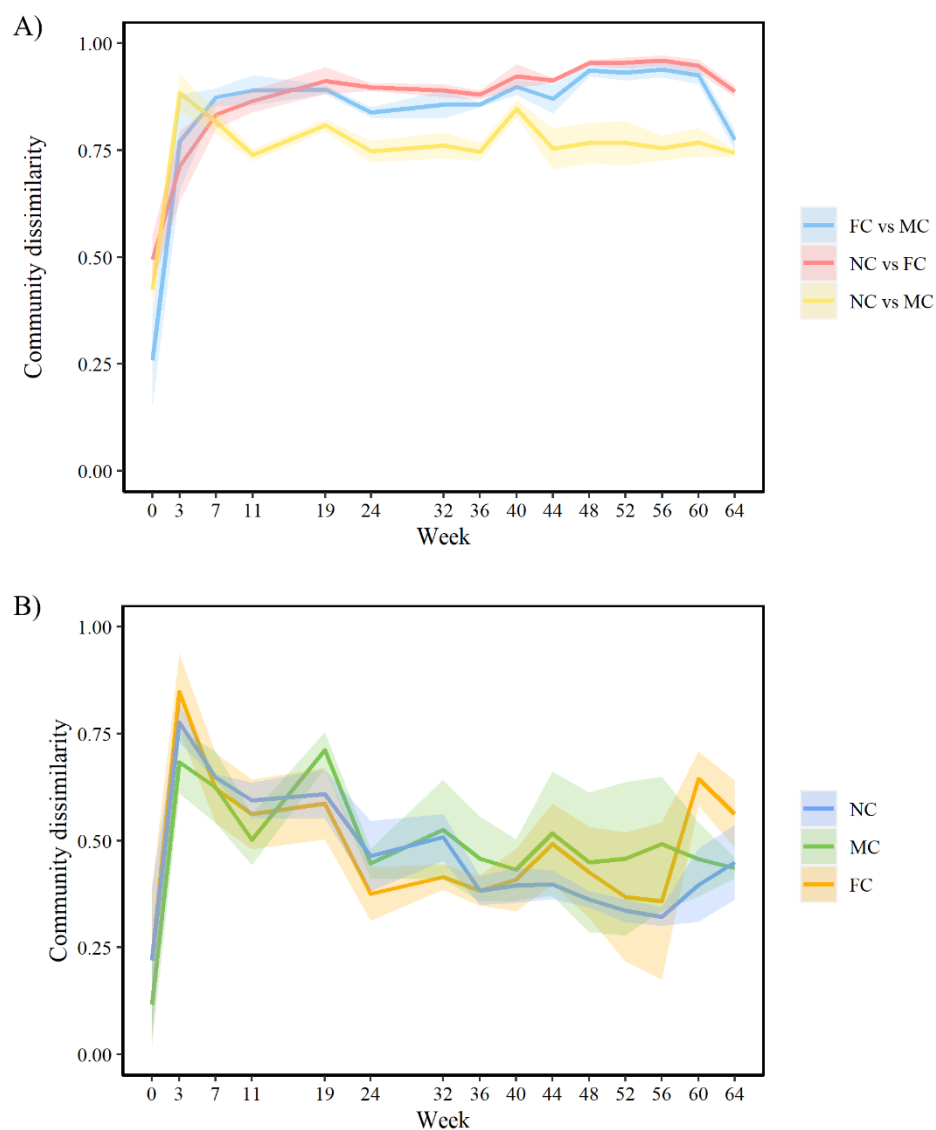
Figure 2-S4. A) Community dissimilarities between biofilm samples collected under different conditions over time based on Bray-Curtis distances; B) Community dissimilarities based on Bray-Curtis distances between two successive sample points under each condition. NC, MC, and FC stand for unchlorinated, monochloramine, and free chlorine applied conditions, respectively. Line plots represent mean values with error bands (mean \pm s.d., n = 3 ).
