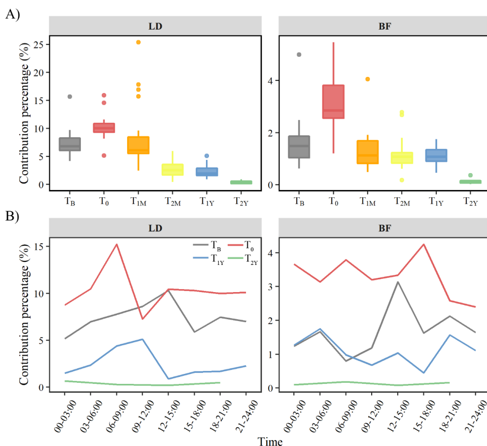
Figure 5-5. Sources apportionment results by SourceTracker2: A) contributions from loose deposits (LD) and biofilm (BF) to particle-associated bacteria (PAB) in distribution network (DN) over time; B) daily variations in contributions from LD and BF to PAB at DN. T B - before introducing RO in production; T 0 - immediately after RO introduction; T 1M - 1 month after RO introduction; T 2M - 2 months after RO introduction; T 1Y - 1 year after RO introduction; T 2Y - 2 years after RO introduction. Box plots show median values (middle line), 25 th and 75 th percentiles (boxes) and 5 th and 95 th percentiles (whiskers). Outliers, if present, are shown as individual points beyond the whiskers.
