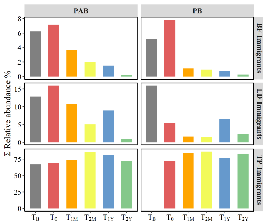
Figure 5-S17. The cumulative relative abundance in immigrants affiliated to particle-associated bacteria (PAB) and planktonic bacteria (PB) from biofilm (BF), loose deposits (LD) and treatment plant (TP) to PAB and PB in distribution network (DN). T B : before the RO introduction; T 0 : immediately after the RO introduction; T 1M : 1 month after the RO introduction; T 2M : 2 months after the RO introduction; T 1Y : 1 year after the RO introduction; T 2Y : 2 years after the RO introduction. TP stands for treatment plant, while DN stands for distribution network.
