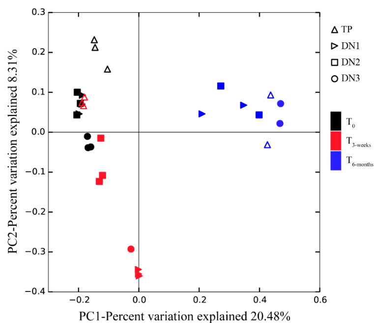
Figure 4-S6. PCoA based on unweighted UniFrac distance for samples taken from treatment plant (TP) to locations in distribution network (DN1, DN2 and DN3) before ( T_0 , black), during ( T_{3\text{-weeks}} , red) and after ( T_{6\text{-months}} , blue) upgrading the treatments were included. The microbial communities of PAB at treatment plant were indicated by open triangles. Communities of PAB during distribution were marked by solid triangles (DN1), squares (DN2), and circles (DN3), respectively.
