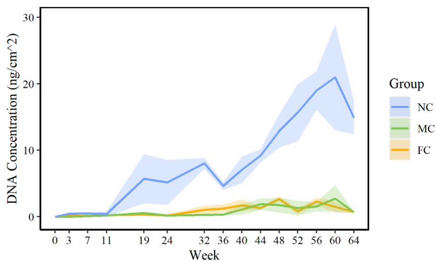
Figure 2-S2. DNA concentration in biofilm under different conditions over the course of the time. Line plots represent mean values with error bands (mean \pm s.d., n = 3 ).
