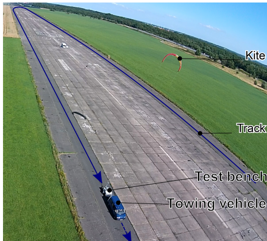
Figure 12. Dynamic test procedure.
