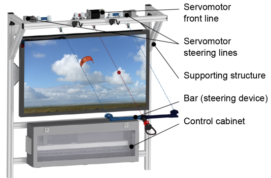
Figure 10. Design of the user interface (bar stand).
