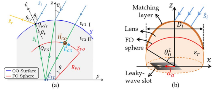
Fig. 2. (a) GO ray propagation for a QO surface. (b) A leaky lens antenna.
