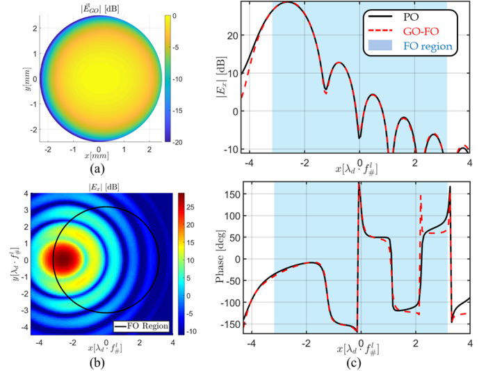
Fig. 3. (a) GO field on the FO sphere. (b) |E_x| calculated by using GO-FO. (c) x-cut of E_x validated by PO for both the amplitude and the phase.
