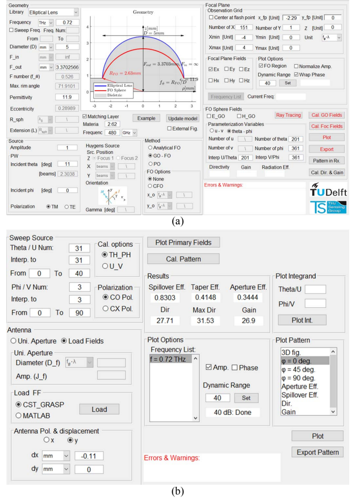
Fig. 1. (a) Main interface. (b) Interface for analyzing reception performance.
