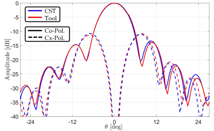
Fig. 4. Co-Pol. ( \phi = 0^\circ ) and Cx-Pol. ( \phi = 45^\circ ) patterns in reception compared to CST simulation.
