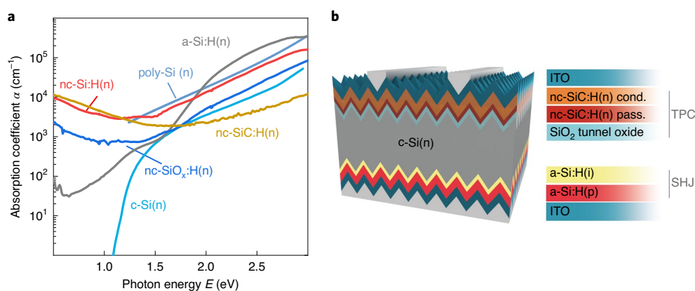
Fig. 1 | Motivation and concept of the TPC. a , The in-house measured absorption coefficient of nc-SiC:H(n), nc-Si:H(n), nc-SiO x :H(n), a-Si:H(n) and poly-Si(n) used in existing passivating contacts. A reference absorption coefficient of c-Si is included 53 . The nanocrystalline silicon/silicon alloys exhibit pronounced free-carrier absorption at low photon energies due to the high doping density. b , Sketch of a silicon solar cell using an n-type wafer with a TPC on front side using our developed nc-SiC:H(n)/SiO 2 stack. Considering the high sheet resistance (approximately 10 6 Ω sq -1 ) of the nc-SiC:H(n), an additional ITO layer with a sheet resistance of approximately 200 Ω sq -1 is used for lateral transport. The back side consists of intrinsic and p-type hydrogenated amorphous silicon (a-Si:H(i/p)) and an ITO layer.
