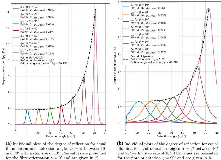
Fig. 6 Plots of the reflectivity for equal incident and detection angles in the interval \beta = [10, 70]^\circ with a step size of 10^\circ . The corresponding Fresnel fittings of the maximum values are visualised
