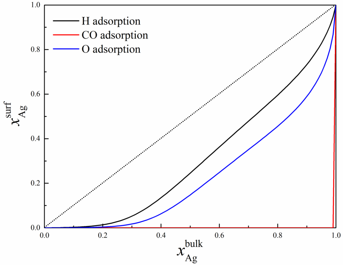
Fig.5 Surface segregation of Pd-Ag alloys with adsorption of different gases at 600 K. The adsorption coverage \theta is also chosen as 1. The no-segregation line, x_A^{\text{surf}} = x_A^{\text{bulk}} , is indicated by the short-dotted line; above this line the solute segregates, below the line Pd segregates.
