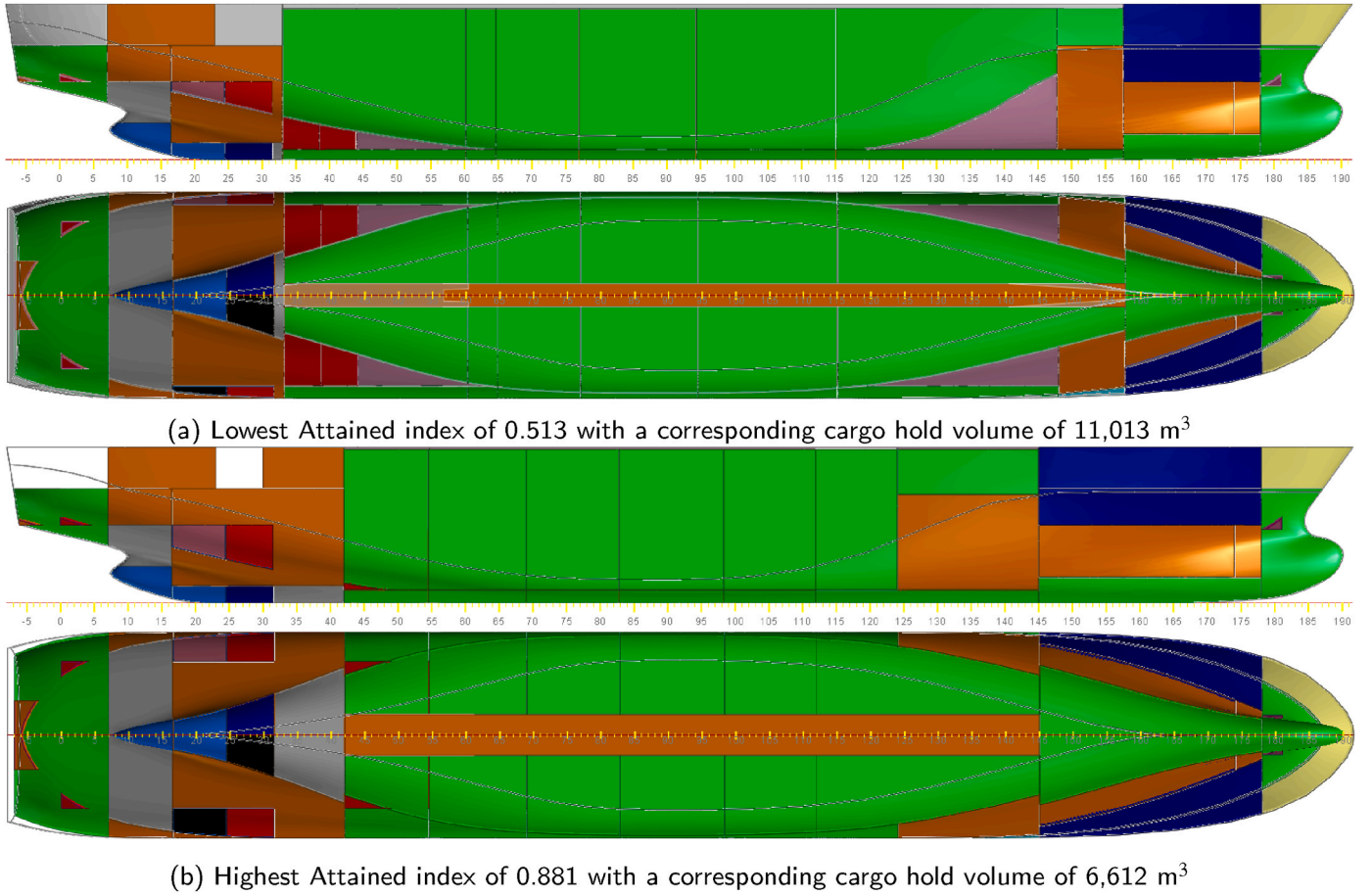
Fig. 11. Extremities of the Pareto front for five water ballast bulkheads.
