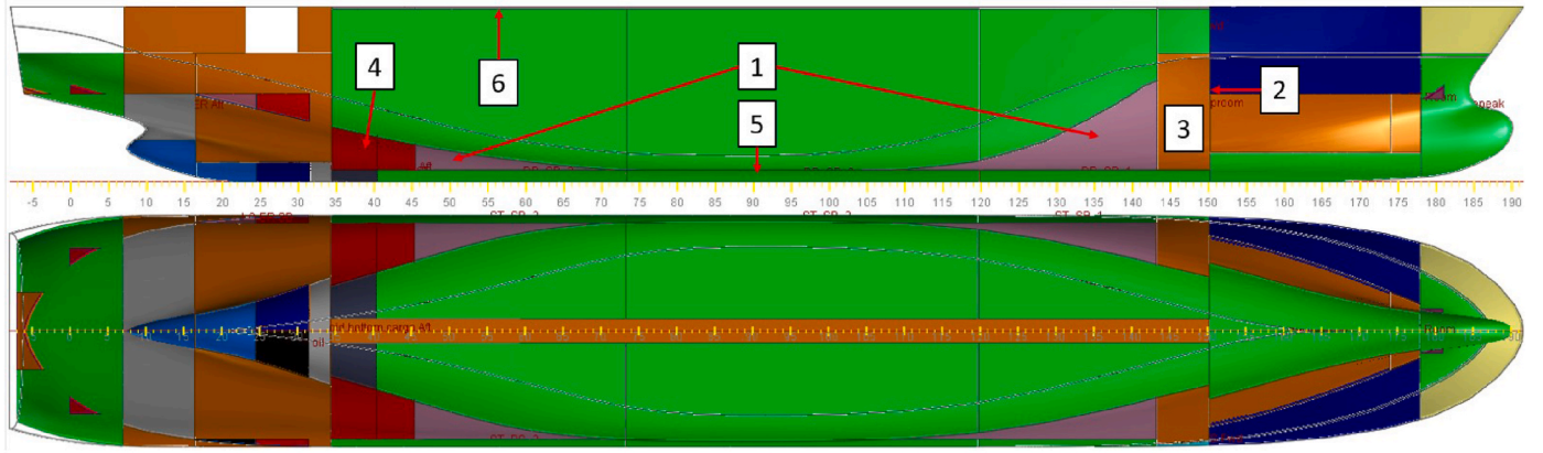
(a) Lowest Attained index of 0.513 with a corresponding cargo hold volume of 10,552 m 3 . Notable properties of the design include: (1) cargo hold is not located within the double bottom, (2) forward cargo hold bulkhead is shifted towards the bow, (3) pump room is at its maximum height and minimum length, (4) fuel oil tanks are higher and more located to the aft, (5) double bottom is at its minimum height, and (6) main deck is at its maximum height.
