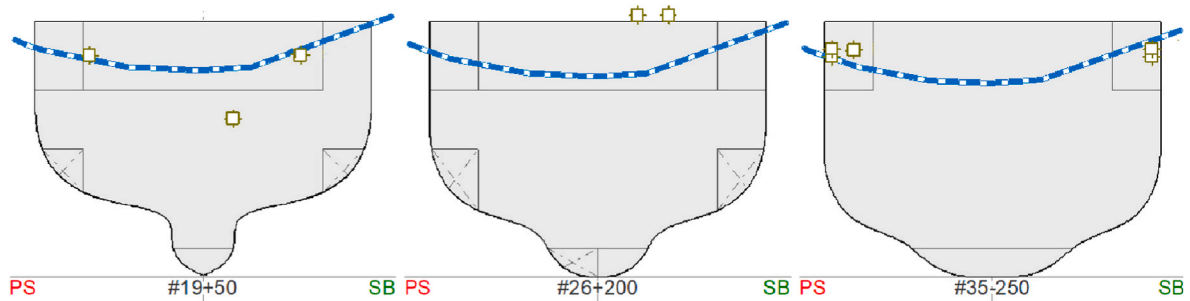
Fig. 8. Damaged waterline (blue/white line) and location of openings (squares) at position zero for different cross sections.
