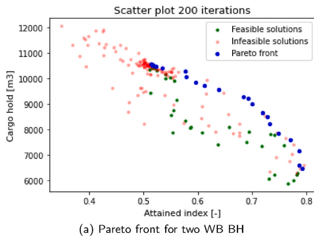
Fig. 6. Scatter plots of the Pareto fronts for two and five water ballast bulkheads (WB BH) investigated designs for 200 iterations.
