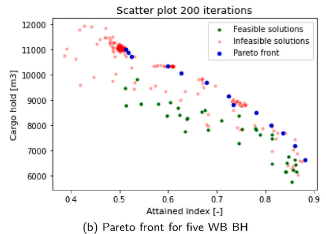
Fig. 6. Scatter plots of the Pareto fronts for two and five water ballast bulkheads (WB BH) investigated designs for 200 iterations.
