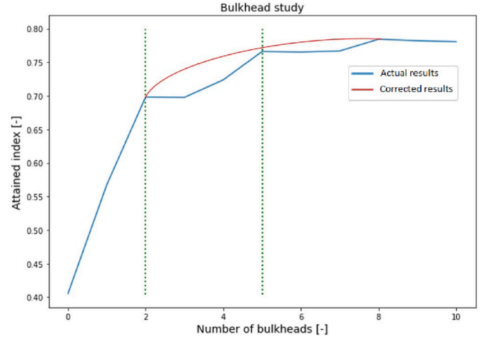
Fig. 4. Results from the first optimisation level.
