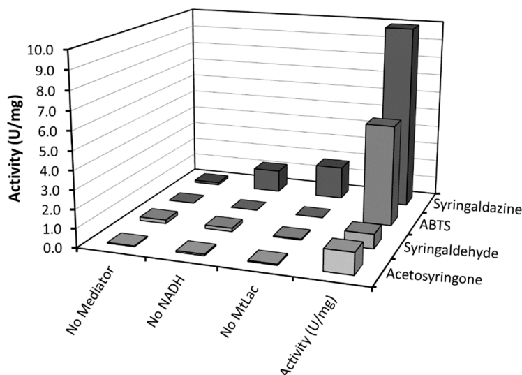
Figure 3. Activity of MtLac in presence of 5 µM of different mediators, 0.5 mM NADH and 100 mM KPi buffer (pH 8.0) at 25 °C. The background activities of the controls in absence of NADH, mediator and laccases are reported.
