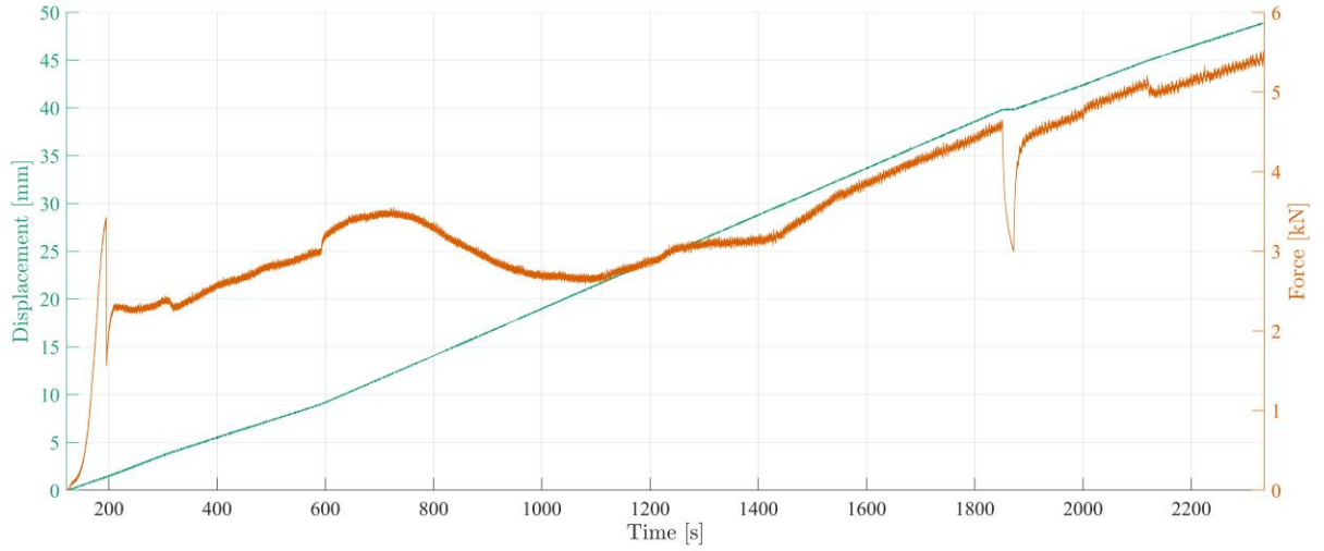
Figure 3. Example time histories of indenter displacement (left) and force (right) for a plane-strain compression of a vertical thick section of S2-type freshwater ice at a nominal strain rate of \dot{\epsilon}_{nom} = 1 \cdot 10^{-4} \text{ s}^{-1} and at an air temperature of -7 \pm 1^\circ\text{C} .
