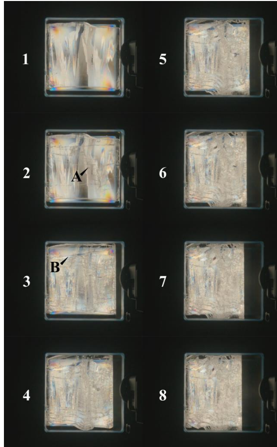
Figure 5. Video frames from the test at time instances corresponding to the labeled markers in Figure 4. The shear fault is labeled A in frame 2. An example of cleavage fracture resulting in a gap in the ice plate is labeled B in frame 3.
