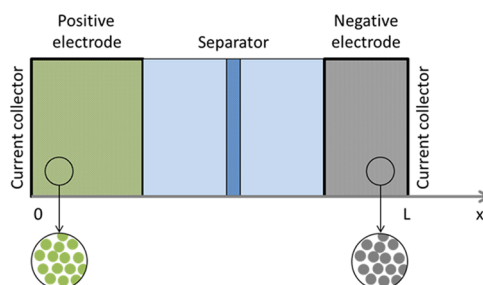
Figure 2. Schematic diagram of battolyser cells and their model representation including the \text{Ni(OH)}_2 positive electrode, aqueous KOH electrolyte, polyphenylene sulfide separator, and \text{Fe(OH)}_2 negative electrode.
