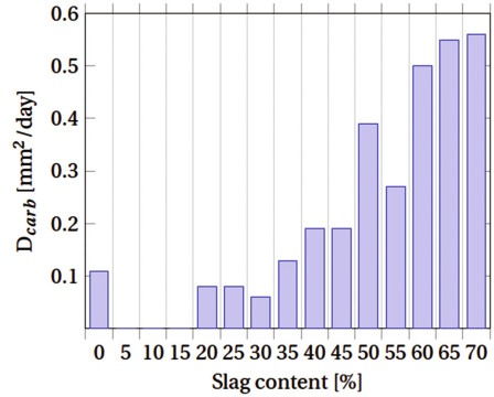
Fig. 3. Carbonation rate, D carb
