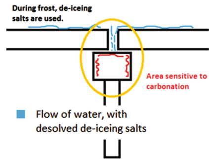
Fig. 1. Sketch of a leaking joint in which de-icing salts coming in contact with underlying carbonated concrete
