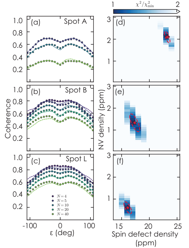
FIG. 5. Simulations of long-lived coherences as in the main text with the color maps, (d), (e), (f) separated instead of superimposed.
