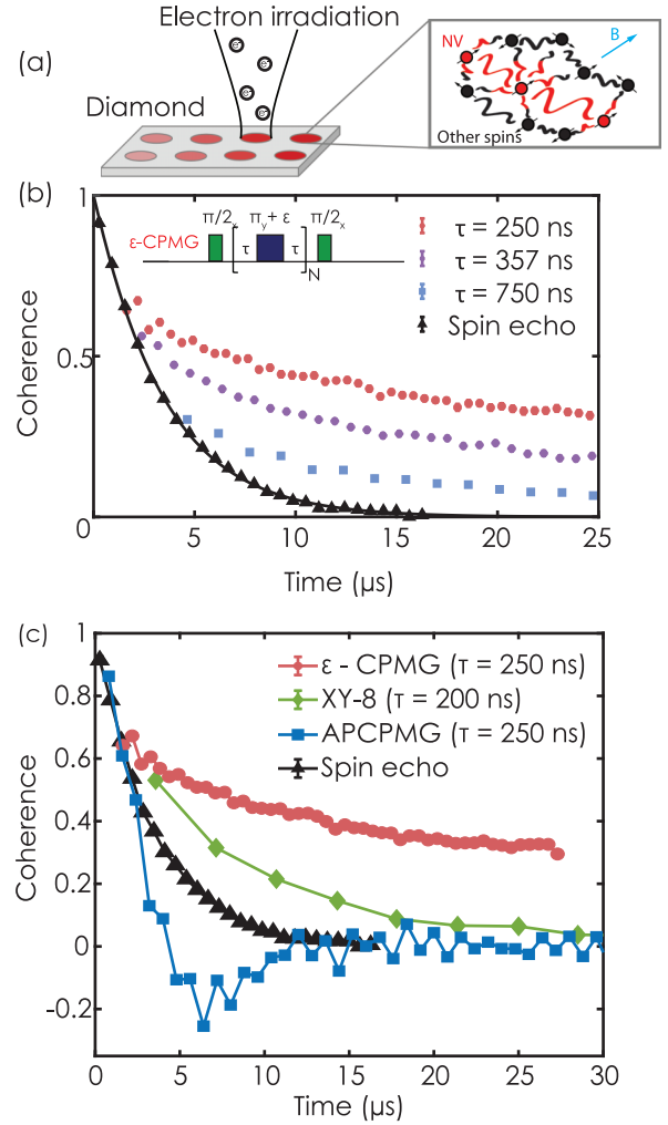
FIG. 1. Measurement of long-lived coherences in a dense NV ensemble. (a) Cartoon sketch of our spin system, a CVD-grown, nitrogen-doped diamond sample showing spots that have undergone localized electron irradiation of varying dosage, resulting in high NV densities that vary across spots. The NV ensemble (red) is mixed randomly with a bath of spins (black). A magnetic field (blue) is applied along the 111 direction. (b) Long-lived coherences observed under \epsilon -CPMG. For the data shown, \theta \approx \pi , and N is varied for various fixed values of \tau . For comparison, the spin echo is also shown ( N = 1 , \theta \approx \pi , variable \tau ). Details of the fit to the spin echo data are given in the Appendices. (c) Comparison of \epsilon -CPMG to APCPMG (which has the same filter function [17–19]) and XY-8, elucidating the importance of a finite \epsilon for preserving coherence in the \epsilon -CPMG sequence ( \tau = 250 ns). Both APCPMG and XY-8 [20] are designed to cancel the effect of accumulating rotation offsets. The experimental data shows a marked difference in coherence between \epsilon -CPMG and the two sequences, reinforcing the notion that the finite, uncontrolled \epsilon in the CPMG sequence is the origin of the state's long-lived nature. The APCPMG coherence decays faster than the XY-8 coherence, likely due to its susceptibility to frequency offsets such as those due to on-site disorder. Even though \epsilon = 0 is targeted in all cases, a finite rotation offset still exists. For reference, a spin echo sequence is shown in black.
