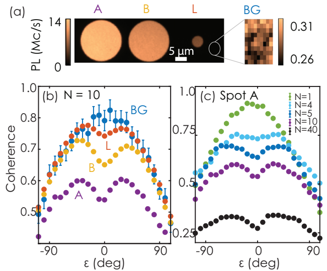
FIG. 2. Behavior of \epsilon -CPMG sequence. (a) Confocal images of spots A, B, and L, showing a range of brightness indicating a range of NV densities. (b) Coherence versus \epsilon for various NV densities at fixed N = 10 and \tau = 250 ns, and (c) for various N for a given NV density (spot A) and \tau . See the Appendices for a comparison of this data to an analytic model.
