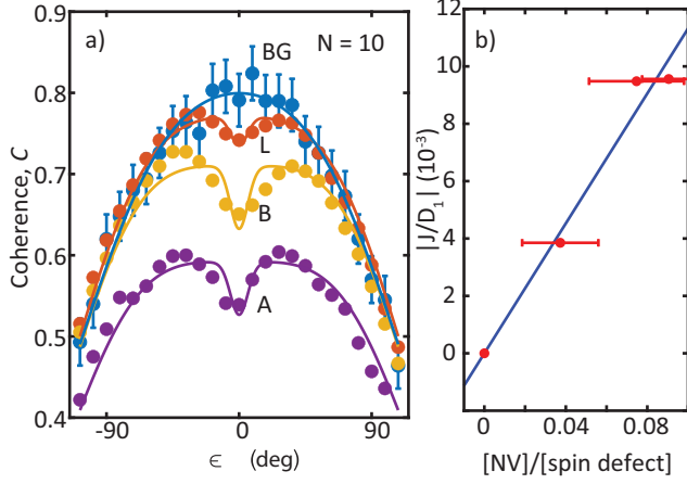
FIG. 4. (a) Comparison of the coherence as a function of \epsilon across different spots to an analytical model that parameterizes the curves in terms of J . (b) A comparison of the fit parameter J/D_1 to the ratio of the NV density to the spin defect density obtained via numerical modeling in the main text. These have the expected linear relationship.
