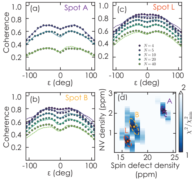
FIG. 3. Simulations of long-lived coherences. (a), (b), (c) Coherence versus \epsilon for various N and for spots A, B, L. Markers show experimental data. Plotted as dashed lines are the numerics for the parameters \{\rho_{NV}, \rho_{bath}\} that minimized \chi^2 . (d) \chi^2 contour plots as a function of \rho_{NV} and \rho_{bath} . The color maps for each spot have been superimposed. Separated colormaps are shown in the Appendices.
