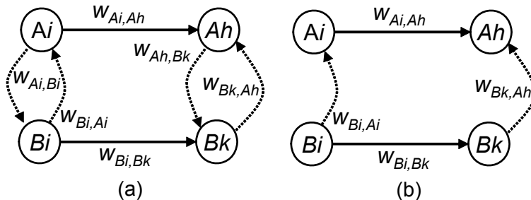
Figure 4: Two aircraft approaching the same air or taxi segment (a) and an ordering decision (b)
