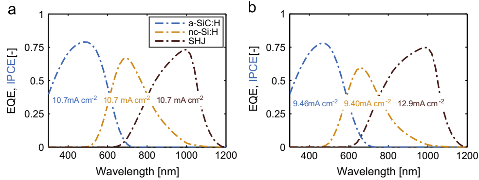
Fig. 4. Simulated IPCE of an a-SiC:H photocathode and EQE of supporting PV stack. (a) Thicknesses used to achieve ideal current matching. (b) Practical thicknesses used.
