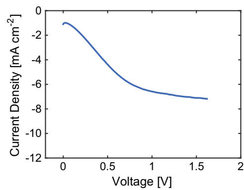
Fig. 3. The J - V curve of an a-SiC:H photocathode as measured with a two-electrode measurement with an \text{IrO}_x counter electrode.
