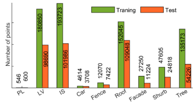
Figure 2. Bar diagrams of the point distribution of the Vaihingen training and test datasets.
