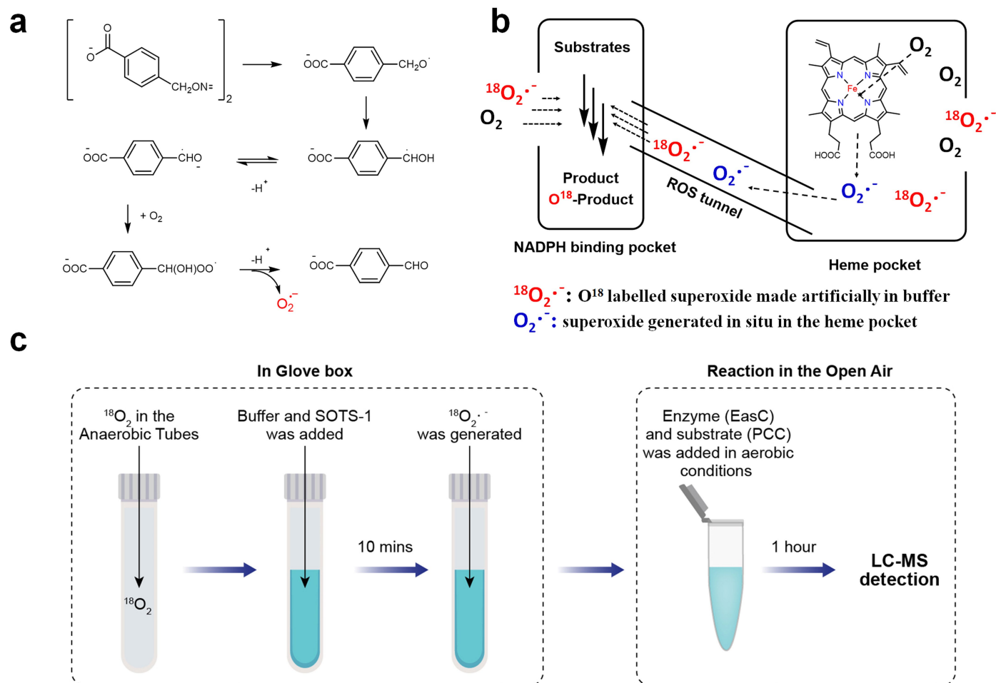
Extended Data Fig. 10 | The competitive incorporation experiment using ^{18}\text{O} -superoxide. a , The pathway for SOTS-1 decomposition and its ensuing reaction with oxygen, leading to the release of superoxide. b , The illustration of the competitive incorporation experiment using ^{18}\text{O} -superoxide in EasC cf reaction. c , The protocol for the artificial production of ^{18}\text{O} -superoxide.
