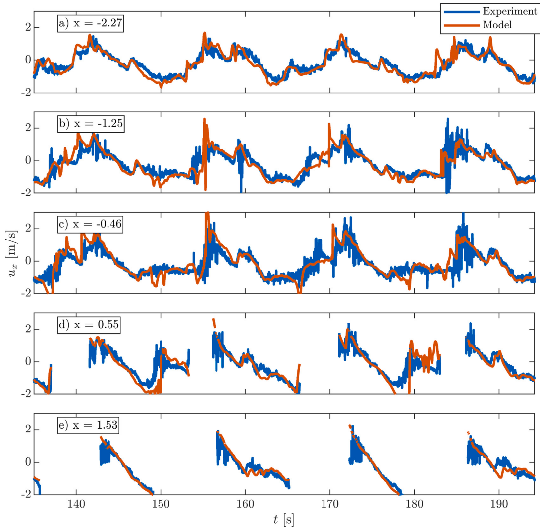
Fig. 9. Comparison between measured and modelled velocities at 3 cm above the bed at five different cross-shore locations, made using model configuration D. In panels (d) and (e) data is omitted when the ADV probe is exposed to air.
