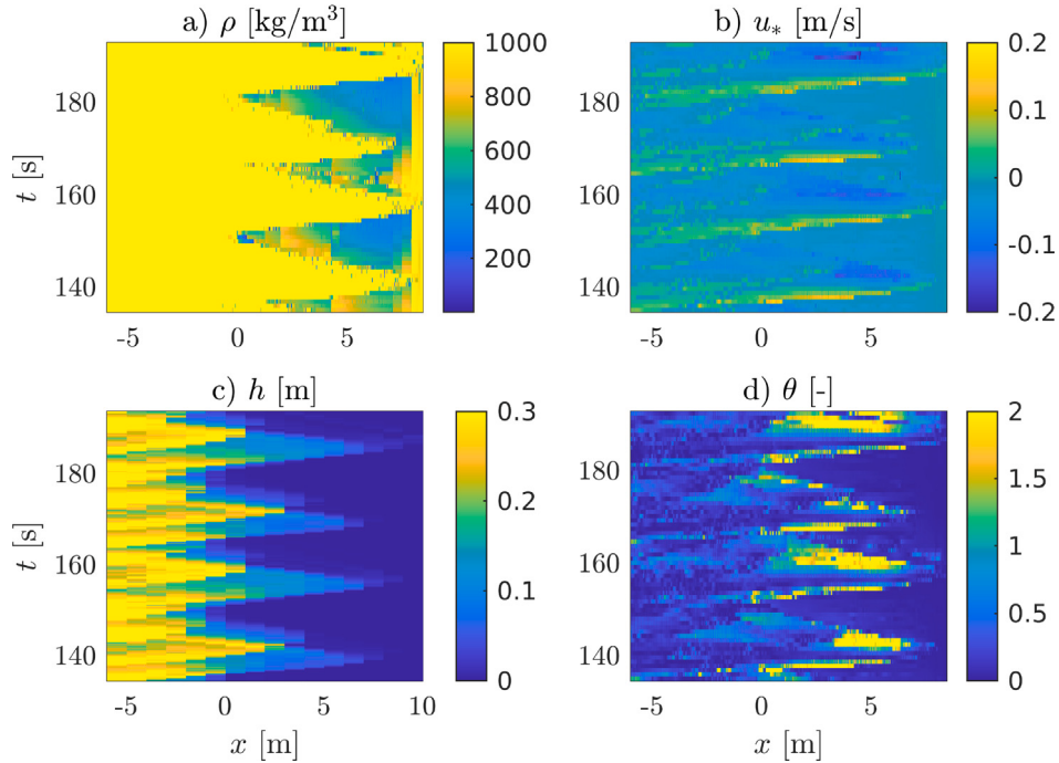
Fig. 4. Time series of the spatial variation in (a) density at the bed, (b) friction velocity u_* , (c) water depth h and (d) Shields parameter \theta from a simulation using Configuration B (Table 1).
