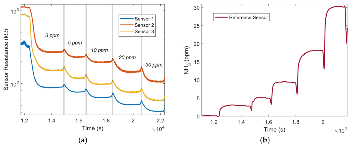
Figure 3. (a) Sensor resistance plotted over time during the calibration experiment. The sensors are exposed to an environment with different concentrations of NH 3 . (b) The reference measurements during the calibration experiment with the calibrated S900 sensor (Aeroqual, New Zealand).
