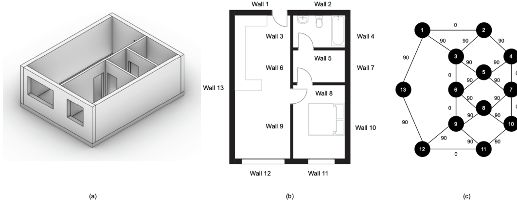
Figure 1. Graph representation of floor plans. (a) 3D model of a floor plan. (b) 2D view showing the wall segments. (c) the graph representation.
