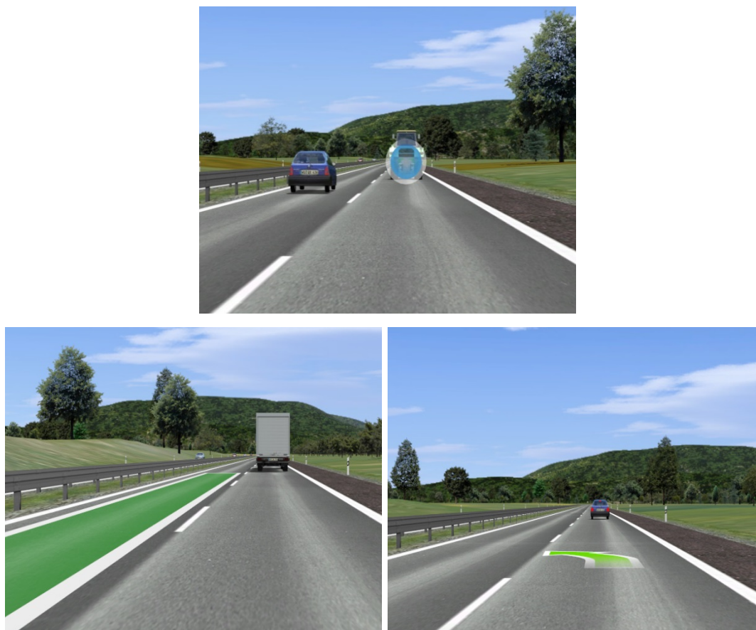
Figure 3. The visual interface in [14]. Top middle (sphere): a sphere highlighting the slow-moving vehicle ahead in both scenarios. Bottom left (carpet): a green carpet in the left lane for the lane change scenario. Bottom right (arrow): a green arrow pointing left for the lane change scenario.
