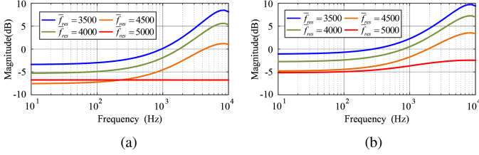
Fig. 4. Bode diagram of the G_V(z) and G_i(z) with different \bar{f}_{res} selections and fixed \delta = 0.8 . f_{res} = 5400 Hz.
