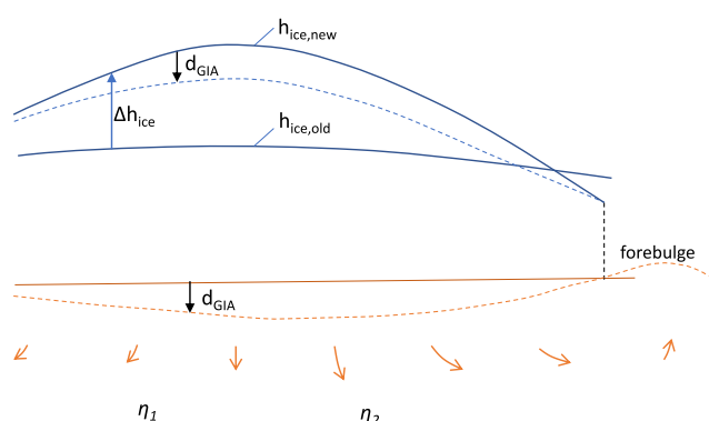
Fig. 1. Schematic representation of GIA following an increase in ice thickness of an ice sheet resting on a bedrock that has two different viscosities. The ice thickness increases by \Delta h_{ice} . As a result of this increase and past increases in ice thickness, the bedrock deforms by d_{GIA} with a forebulge forming outside the area of ice increase. Because viscosity \eta_2 is assumed to be smaller than \eta_1 , deformation is larger under the right half of the ice sheet in a given time.
