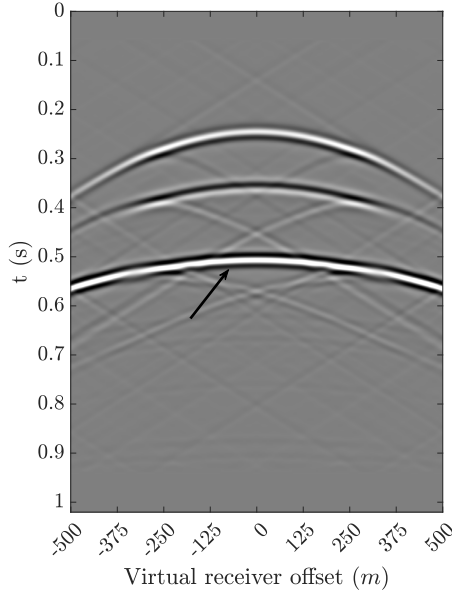
Figure 3.4.: Upgoing component of data at the upper boundary with a source located at \mathbf{x}_s = (0,0) . This is the data corresponding to the first term on the right-hand side of Equation 3.17. The black arrow indicates the total event generated by the reflector below the target region described by the left-hand side of Equation 3.15.
