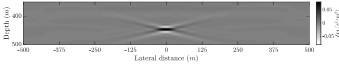
(b) LSRTM
