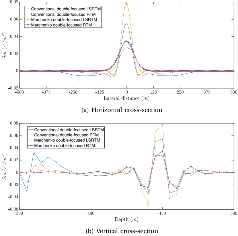
Figure 2.9.: A comparison of the horizontal and vertical cross-section of the retrieved image of the simple model with different approaches. a) A horizontal cross-section at depth of 450 m, and b) A vertical cross section at lateral distance zero.
