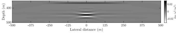
(a) RTM
