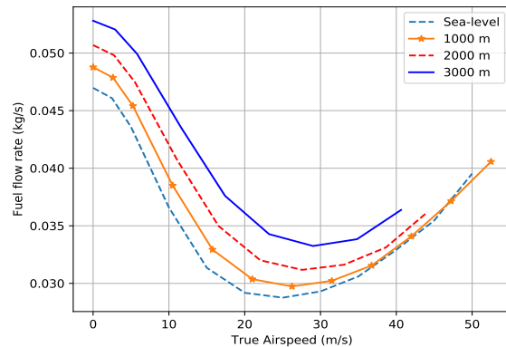
Figure 18: Fuel flow rate vs Airspeed for Bo105 at various flight altitudes
