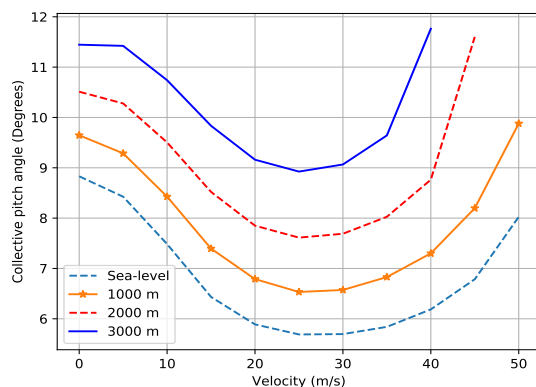
Figure 19: Collective pitch vs Airspeed for B0105 at various flight altitudes
