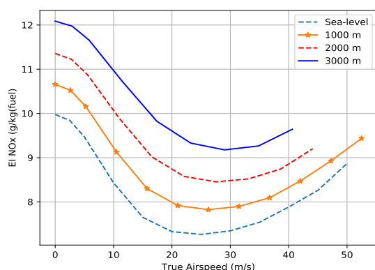
Figure 17: Engine Emission vs Airspeed for Bo105 at various flight altitudes
