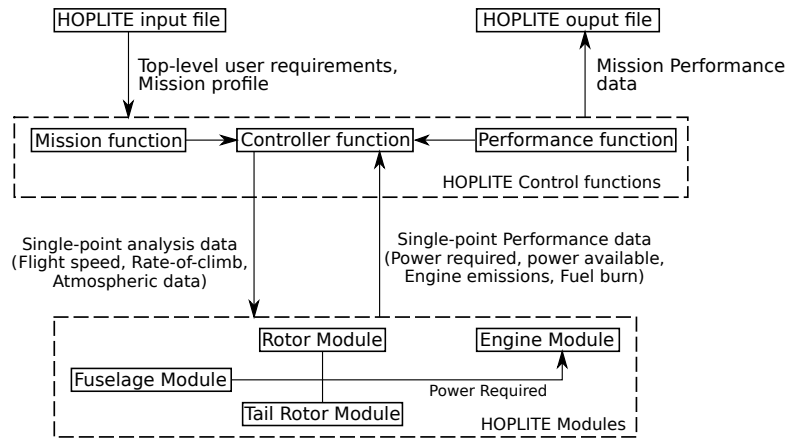
Figure 14: Workflow of HOPLITE in Analysis mode
