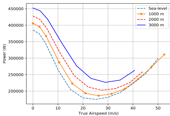
Figure 16: Power required vs Airspeed for Bo105 at various flight altitudes
