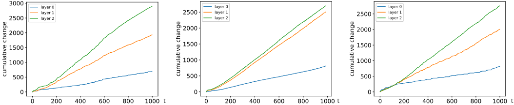
Figure 13: Absolute cumulative change in the attention masks for three different models on Walker-7.
