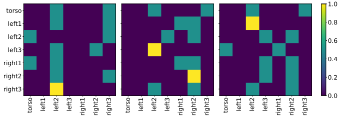
Figure 5: State-dependent masks of AMORPHEUS (3 rd attention layer) within a Walker-7 rollout.
