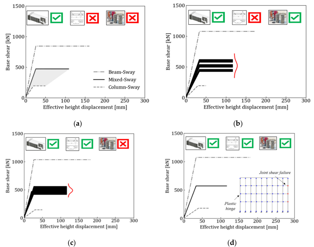
Figure 19. SLA-based pushover capacity curves for all case-study scenarios: Scenario 1 (a), Scenario 2 (b), Scenario 3 (c), and Scenario 4 (d).
