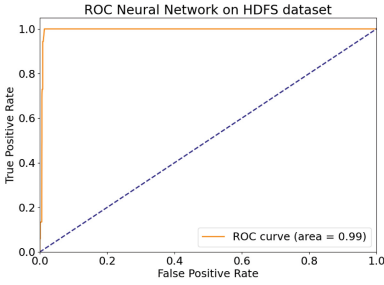
(c) HDFS dataset: Network.
