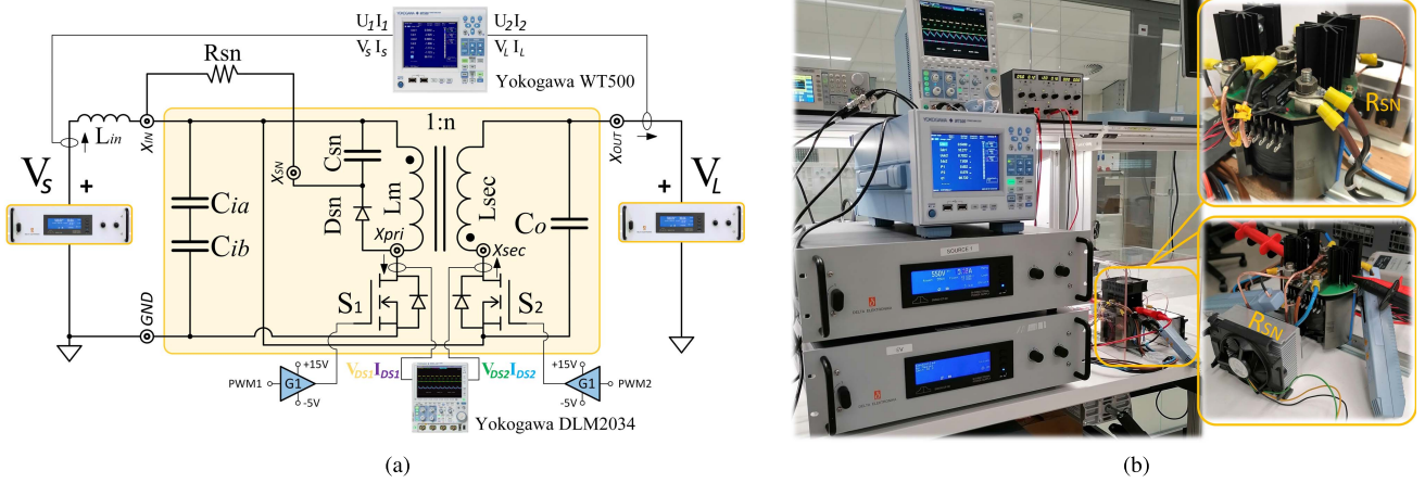
Fig. 10. Measurements setup. (a) Setup drawing. (b) Setup picture.
