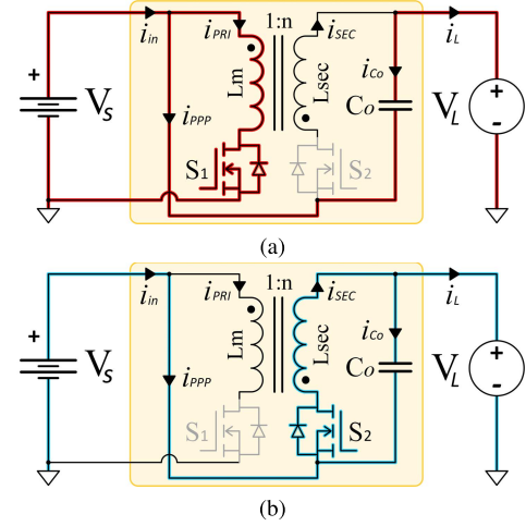
Fig. 5. Bidirectional series PPP flyback topology current conduction subintervals. (a) D subinterval. (b) D' subinterval.
