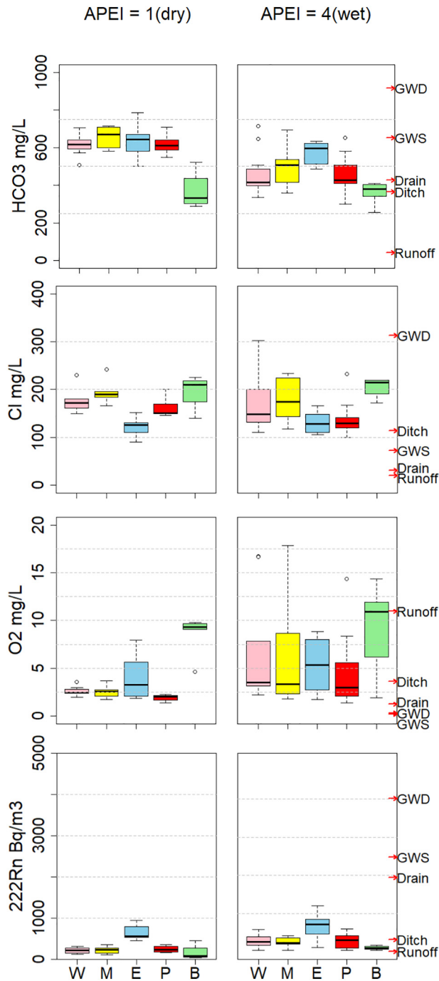
Fig. 5. Summary of the measured \text{HCO}_3^- , \text{Cl}^- , \text{O}_2 , ^{222}\text{Rn} , and \text{pCO}_2 concentrations in the surface water aggregating the 2016–2017 data for dry periods (APEI class = 1) and wet periods (APEI class = 4). The locations of W, M, E, and B represent the total of measurements in the West ditch, the Middle ditch, the East ditch and boezem water north of Geuzenveld, respectively. “P” represents the measurements at the pumping station. Red arrows are used to illustrate the median concentrations that were observed in the 2017 spatial survey (see Section 3.1 and Fig. 3). GWD: deep groundwater, GWS: shallow groundwater, Drain: drain water, Ditch: ditch water, Runoff: rain water.
