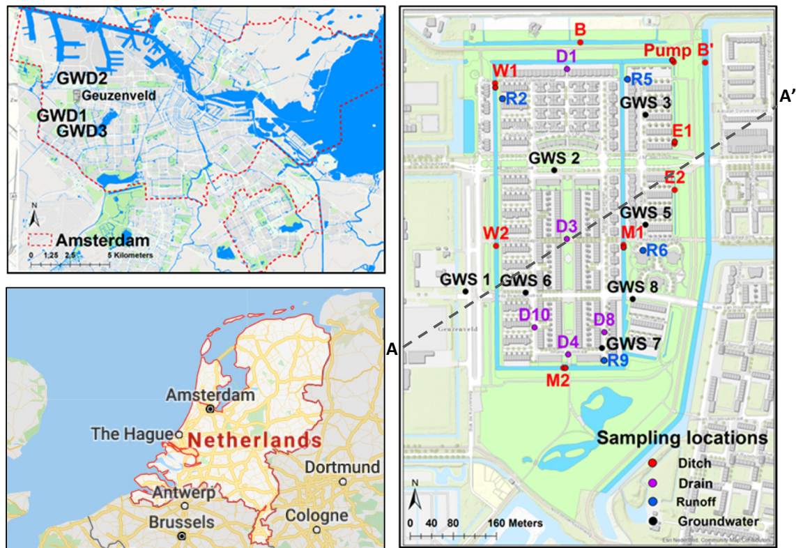
Fig. 1. Location of polder Geuzenveld ( 52^{\circ}23'01.3''\text{N} 4^{\circ}47'37.7''\text{E} ) in the greater Amsterdam area (left figure) and detailed map of Geuzenveld (right figure). The Amsterdam map shows the location of polder Geuzenveld and the deep groundwater sampling locations (GWD1, GWD2 and GWD3). The Geuzenveld map shows the sampling locations of the short term (2016–2017) grab sampling (W1, W2, M1, M2, E1, E2, B, and B'), the water quality survey in 2017 of runoff (R2, R5, R6, and R9), ditch (W1, M1, M2, E1, and Pump) and drain water sampling manholes (D1, D3, D4, D8, D10) and shallow groundwater piezometers (GWS 1–3, GWS 5–8).
