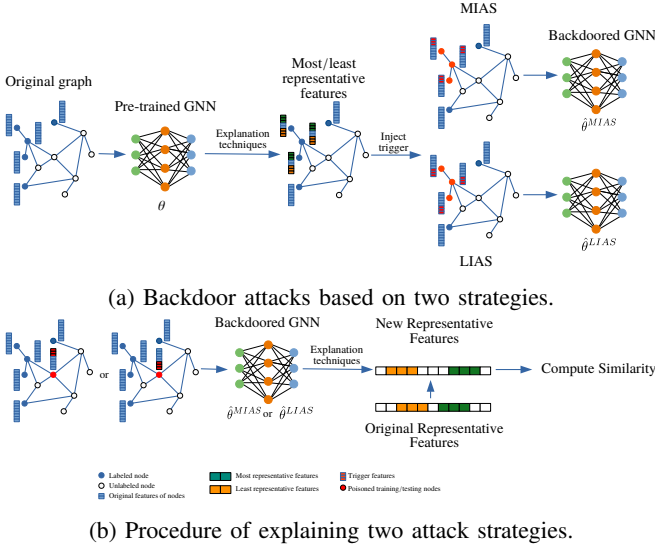
Fig. 2: An illustration of backdoor attack and explanation framework.
