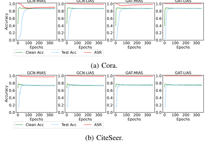
Fig. 3: Backdoor attack results of two trigger-injecting strategies.
