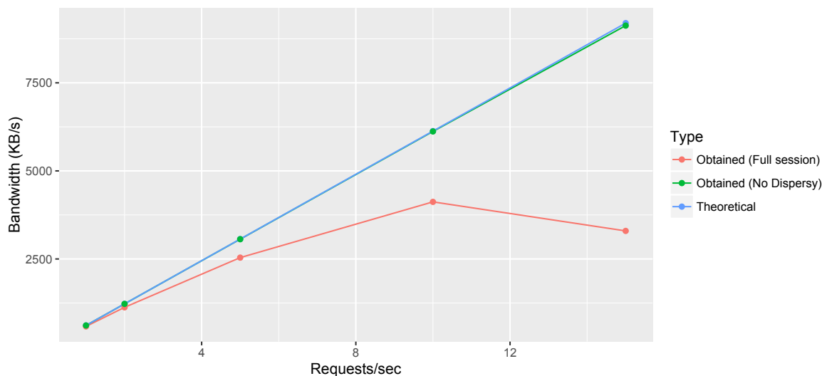
Figure 6.5: The theoretical maximum bandwidth compared to the observed bandwidth in the experiments (using a full Tribler session and disabled Dispersy).
