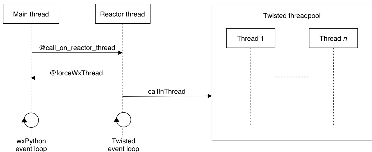
Figure 3.4: The threading model used by Tribler 6, together with the primitives to schedule operations on different threads.
