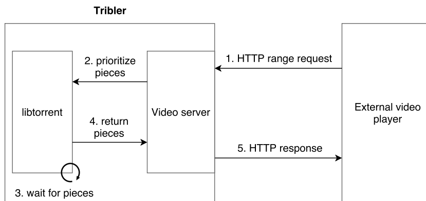
Figure 3.7: The sequence of operations when performing a HTTP range request when streaming a video using Tribler.
