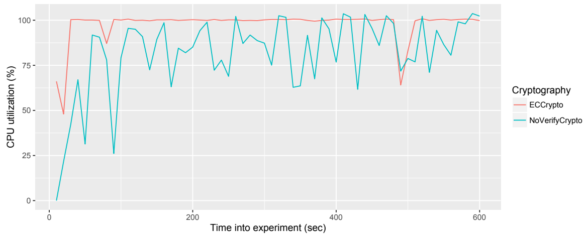
Figure 6.2: The CPU utilization of one core on a Raspberry Pi device when running Tribler with and without cryptographic verification of incoming Dispersy messages.
