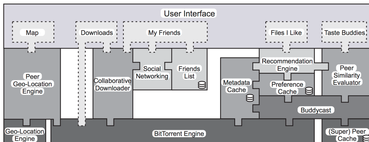
Figure 3.1: The system architecture of Tribler in 2007 as described in [44].
