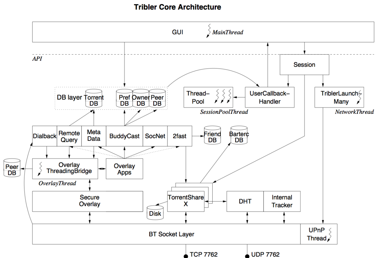
Figure 3.3: An overview of the core architecture around the time of Tribler 5.5.
