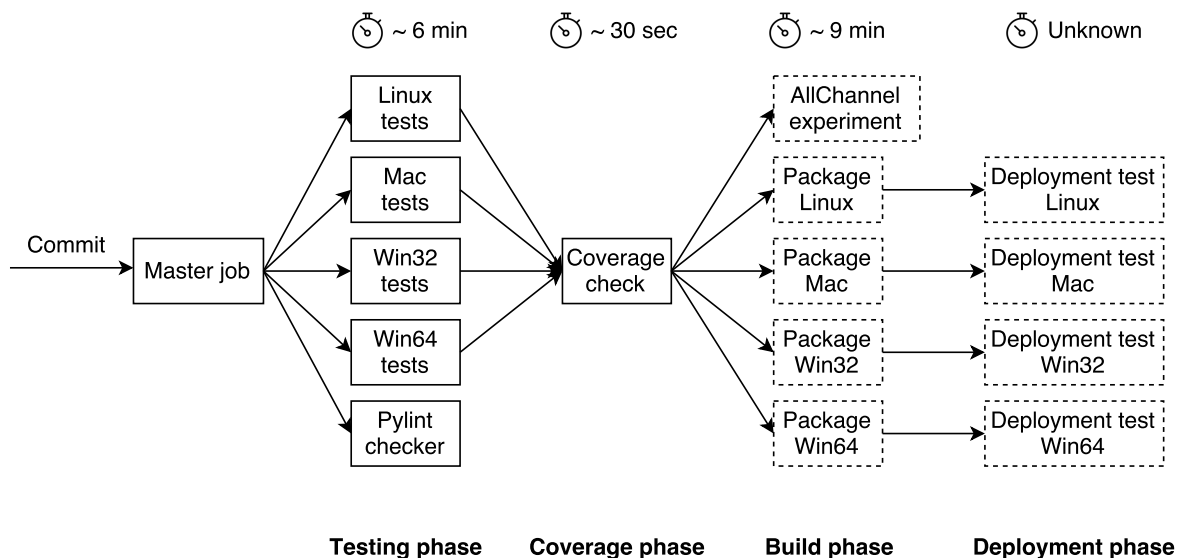
Figure 5.7: The desired test execution plan in our CI environment. Dashed boxes are Jenkins jobs that are not implemented yet.
