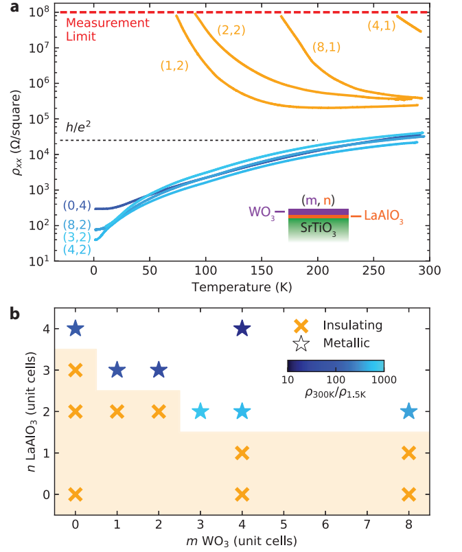
FIG. 2. Insulator-to-metal transition in \text{WO}_3/\text{LAO}/\text{STO} heterostructures. (a) Resistance versus temperature for different (m, n) thickness combinations and (b) transport phase diagram showing insulating (orange cross) and metallic (stars with colour scale) heterostructures. The colour scale indicates the residual-resistance ratio for the metallic samples and the orange shaded area marks the (m, n) combinations constituting insulating heterostructures.
