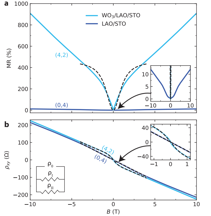
FIG. 3. Comparison of \text{WO}_3/\text{LAO}/\text{STO} and \text{LAO}/\text{STO} magnetotransport. (a) Magnetoresistance and (b) Hall effect measured at 1.5 K in Van der Pauw geometry, with respective zoom-in (insets). The Hall data is fitted (dashed lines) with eq. (1b) and used to extract the values in table I. The classical MR (dashed line in (a)) is calculated from these value using eq. (1a).
