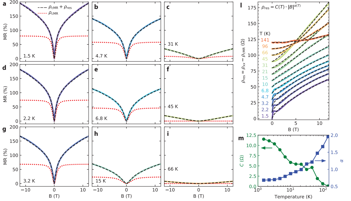
Supplementary Figure 5. Phenomenological magnetoresistance fits. (a) to (i) Experimental magnetoresistance (solid line) at different temperatures, classical magnetoresistance \rho_{\text{cMR}} (red dotted line) calculated with the parameters extracted from the Hall effect and total magnetoresistance (black dashed line), obtained summing the residual magnetoresistance fit \rho_{\text{res}} with \rho_{\text{cMR}} . (j) Residual magnetoresistance curves (offset for clarity) are fitted with a power law function (dashed black lines) and the extracted parameters are in (k). The fits, performed in the 3 T to 12 T range, well represent the high-field part of the experimental curves. A decreasing trend as a function of temperature is found for the amplitude factor C(T) , consistent with the decreasing magnetoresistance effect. The exponent \alpha(T) , instead, grows with increasing temperature and passes from \alpha < 1 ( \rho_{\text{res}} curve concave down) to \alpha > 1 ( \rho_{\text{res}} concave up) at about 30 K. We note that this temperature corresponds to the crossover from two to one conduction channels observed in the Hall measurements. The power-law dependence of this residual magnetoresistance might be related to spatial inhomogeneities of n_{2D} , \mu or disorder.
