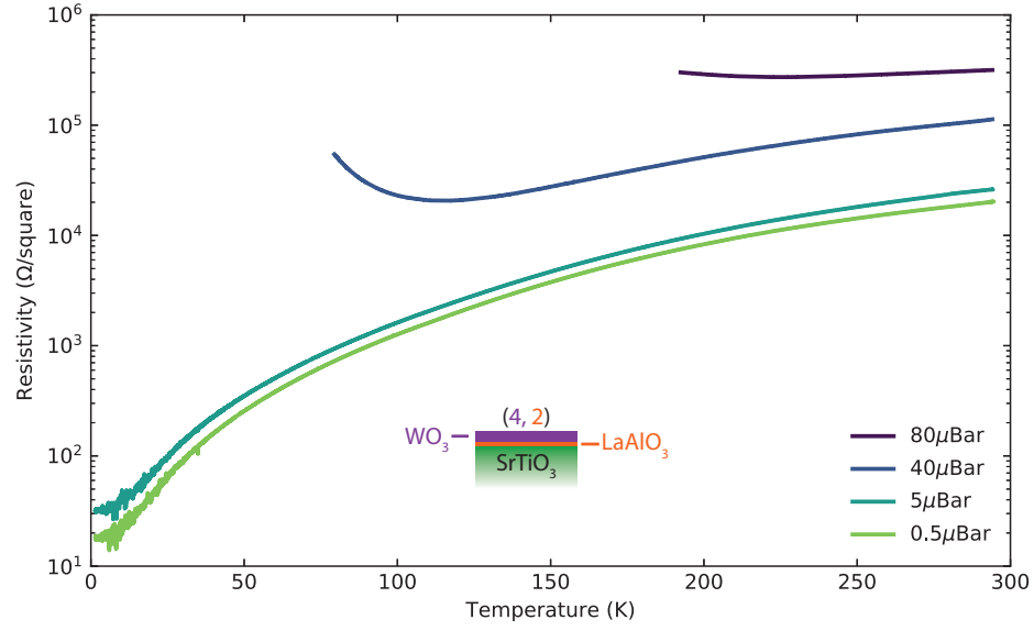
Supplementary Figure 3. Transport of a (4, 2) \text{WO}_3/\text{LAO}/\text{STO} heterostructures where \text{WO}_3 is grown in different oxygen pressures. We measure the metallic trend discussed in the paper only when the \text{WO}_3 overlayer is grown in a low oxygen pressure ( p_{\text{O}_2} < 40 \mu\text{bar} ). This shows the important role of defect formation, such as oxygen vacancies, in the \text{WO}_3 overlayer in order to obtain the enhanced 2DES at \text{WO}_3/\text{LAO}/\text{STO} heterostructures.
