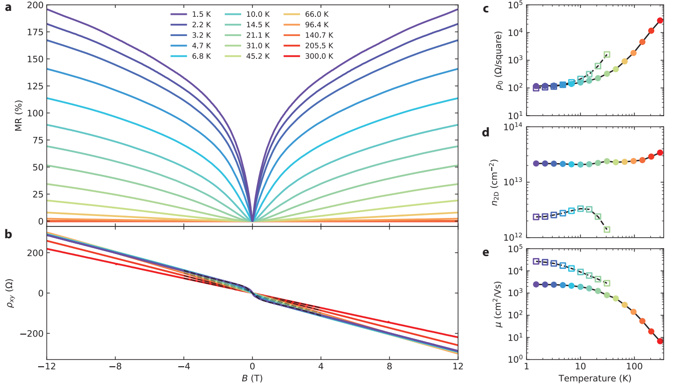
Supplementary Figure 4. Temperature dependent magnetotransport of a (4,2) \text{WO}_3/\text{LAO}/\text{STO} heterostructure. (a) Magnetoresistance and (b) Hall effect measured at different temperatures in a Hall bar configuration. Fits of the Hall effect curves allow to extract (c) sheet resistance, (d) carrier density and (e) mobility of the multiple conduction channels.
