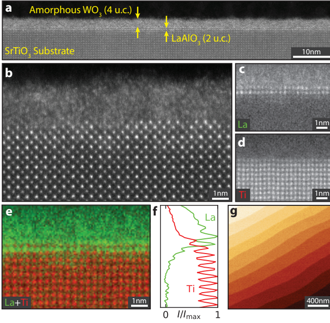
FIG. 1. Structural characterisation of \text{WO}_3/\text{LAO}/\text{STO} heterostructures. (a) Lower magnification and (b) close-up HAADF-STEM image from a (4,2) heterostructure along the (001) direction. (c) EELS elemental map showing normalized core-loss signals for La- M_{4,5} , (d) Ti- L_{2,3} edges and (e) combined signal. (f) Normalised EELS intensity profile averaged along the direction perpendicular to the interface. (g) Surface topography by AFM.
