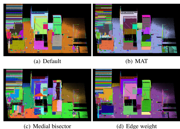
Figure 8. SynthCity geometric partition comparison.
