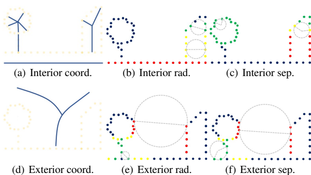
Figure 3. 3D medial axis transform (MAT) as a point feature. Here, ‘coord.’ represents coordinates (a 3D feature vector), ‘rad.’ denotes radius (a scalar feature value), and ‘sep.’ stands for separation angle (also a scalar feature value). Colors in (b), (c), (e), (f) indicate scalar feature values from low to high, and the interior and exterior shrinking balls are represented by gray dashed lines.
