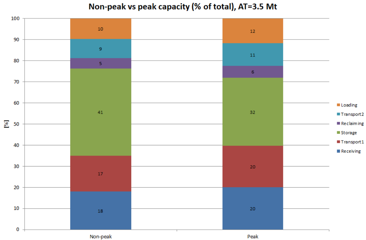
Figure 4.7: Non-peak vs peak capacity cost breakdown (3.5 Mt throughput terminal)
