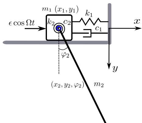
Fig. 8 A pendulum slider under periodic forcing
