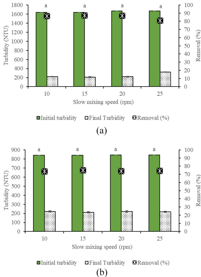
Fig. 8. Influence of SMS to (a) artificial wastewater and (b) aquaculture effluent treatment. Values shown are mean \pm SD. Same letters above the graph (a) indicate no significant differences in turbidity removal between SMS based on ANOVA ( p > 0.05 ).
