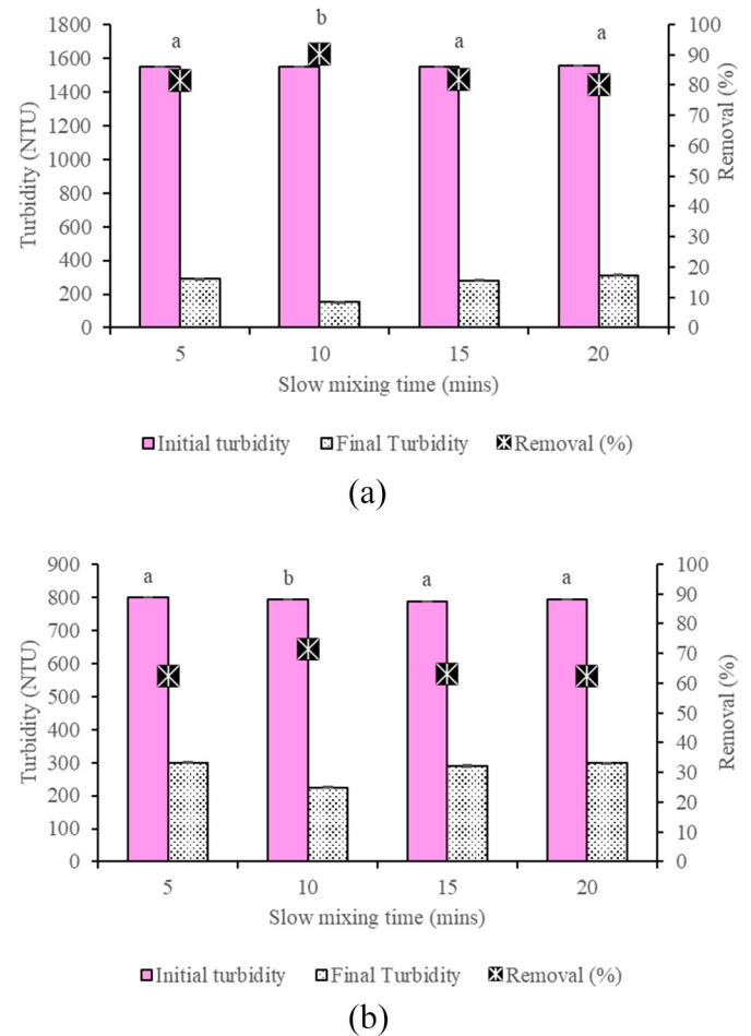
Fig. 9. Influence of SMT to (a) artificial wastewater and (b) aquaculture effluent treatment. Values shown as mean \pm SD. Different letters above the graph (a-b) indicate significant differences in turbidity removal between SMT based on ANOVA ( p \leq 0.05 ).
