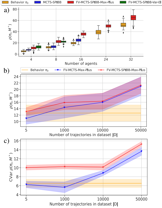
Figure 2. Multi-agent SysAdmin with ring topology: performance. a) Scalability of FV-MCTS-SPIBB (Max-Plus and Var-El): performance as the number of agents increases. b, c) Safety of FV-MCTS-SPIBB-Max-Plus ( \bar{\rho}(\pi, M^*) and CVaR) as the number of trajectories increases. Results obtained using Var-El instead of Max-Plus in the Supplementary Material.
