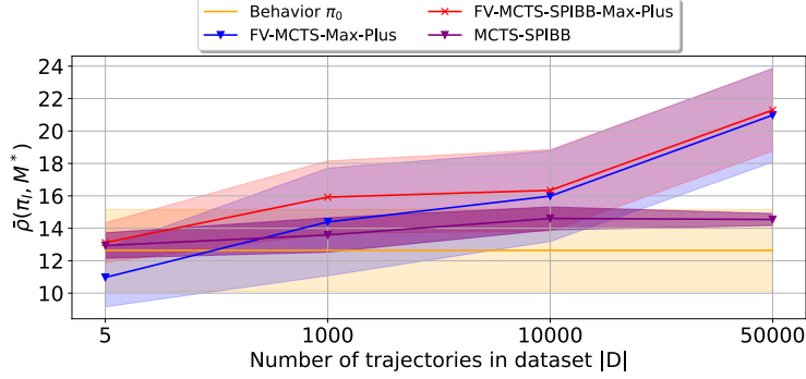
Figure 7. Multi-agent SysAdmin with ring topology: a) comparison on sample efficiency of FV-MCTS-SPIBB-Max-Plus (our method, red line), FV-MCTS-Max-Plus (Choudhury et al., 2021) (blue line) and MCTS-SPIBB (Castellini et al., 2023) (purple line) measured in terms of performance \hat{\rho}(\pi, M^*) as the number of trajectories increases.
