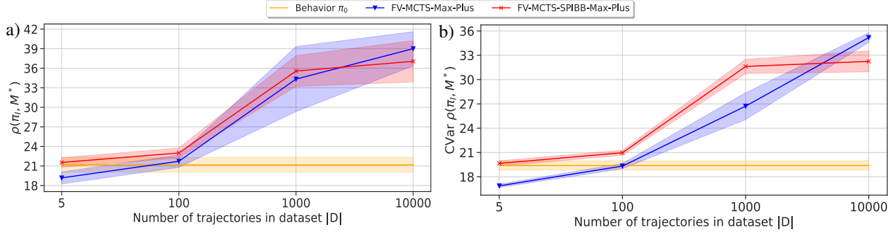
Figure 10. Multi-agent SysAdmin with star topology: performance. a, b) Safety of FV-MCTS-SPIBB-Max-Plus ( \bar{\rho}(\pi, M^*) and CVaR) as the number of trajectories increases.
