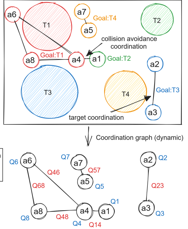
Multi-UAV Delivery, 8 agents
