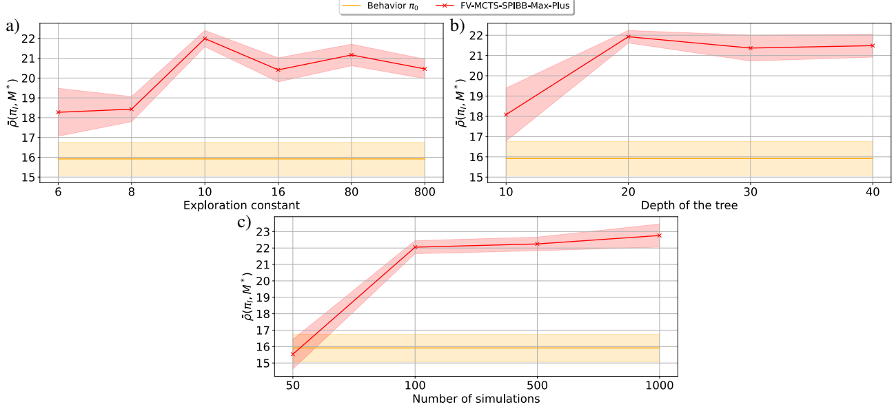
Figure 6. Multi-agent SysAdmin with ring topology: ablation study on the sensitivity of MCTS parameters, namely: a) on the UCT exploration constant; b) on tree depth of MCTS; c) on the number of simulations.
