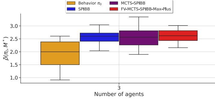
Figure 8. Multi-agent SysAdmin with ring topology: additional results of baseline SPI methods on multi-agent SysAdmin with 3 agents.
