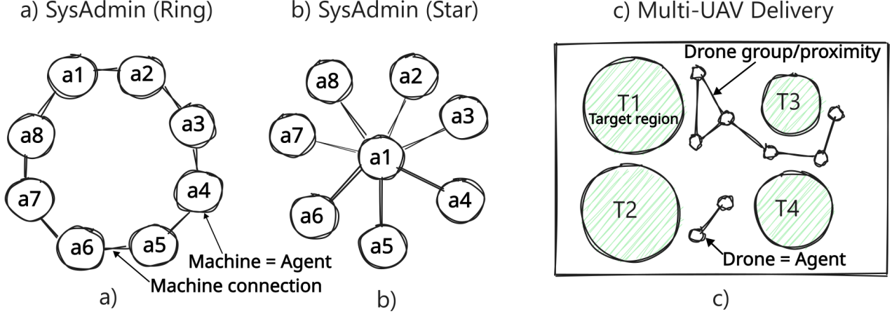
Figure 5. Domains. a,b) Multi-agent SysAdmin with ring/star topology (static and cyclic/acyclic coordination graph); c) multi-UAV Delivery (dynamic and cyclic coordination graph).
