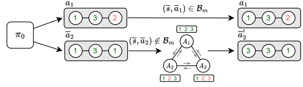
Figure 1. Action selection strategy (Algorithm 2). A synthetic example with three agents (circles), each one with three local actions. In this case, an agent corresponds to a factor. In red “bootstrapped” local actions (i.e., n_{\mathcal{D}}(D_k(\bar{s}, \bar{a})) < m_k ), in green “non-bootstrapped” local actions. On top: a “bootstrapped” local action makes the joint action \bar{a}_1 bootstrapped, so it is returned as it is; at the bottom, only “non-bootstrapped” local actions have been selected so \bar{a}_2 is also non-bootstrapped: the agents communicate via message-passing to compute and return the best non-bootstrapped joint action.
