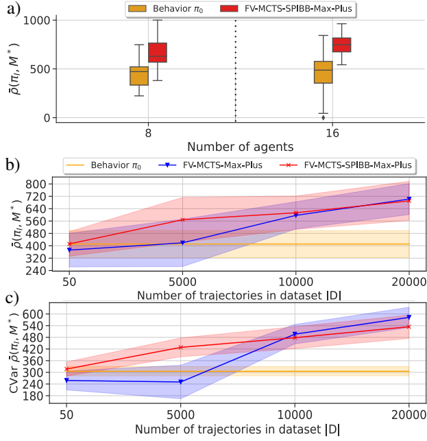
Figure 3. Multi-UAV Delivery: performance. a) Scalability of FV-MCTS-SPIBB-Max-Plus: performance as the number of agents increases. b, c) Safety of FV-MCTS-SPIBB-Max-Plus as the number of trajectories increases.
