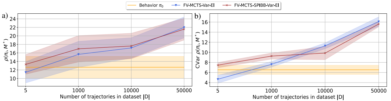
Figure 9. Multi-agent SysAdmin with ring topology: performance. a, b) Safety of FV-MCTS-SPIBB-Var-El ( \bar{\rho}(\pi, M^*) and CVaR) as the number of trajectories increases.
