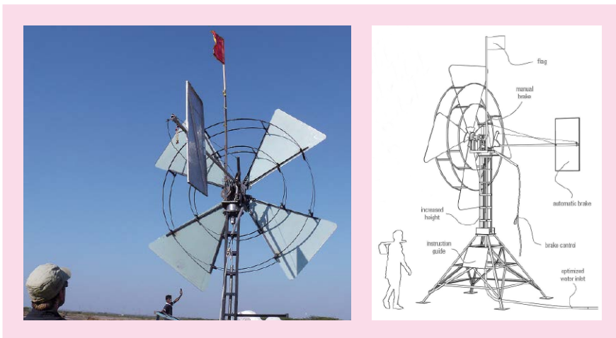
Figure 3.20 The flag on the redesigned windmill [case 2.11], designed by Casper van der Meer, Emma Haagen, Juan David Martin and Nick van der Velde (2012)
