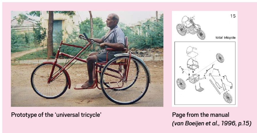
Figure 1.8 A prototype of the 'universal tricycle' and a page from the tricycle-production manual
