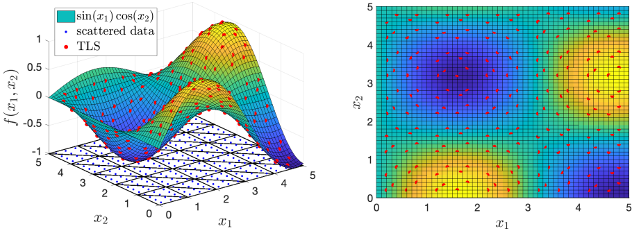
Figure 6.7: TLS reconstructions of f(x_1, x_2) = \sin(x_1) \cos(x_2) on [0, 5] \times [0, 5] using 30 triangular elements with 6 data points within each element. The TLS reconstruction is evaluated at Gauss-point positions within each element.
