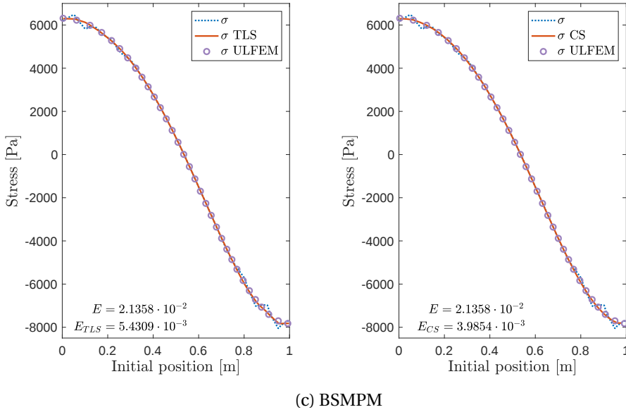
Figure 5.13: Stress distribution and corresponding relative errors in the L_2 -norm in the vibrating bar problem with grid crossing. The results are obtained for BSMPM without reconstruction technique, with cubic-spline reconstruction (CS) and TLS reconstruction, and are compared to the ULFEM results.
