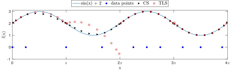
Figure 5.5: Comparison of the cubic-spline and TLS reconstructions of f(x) = \sin(x) + 2 on [0, 4\pi] for a challenging local data distribution.
