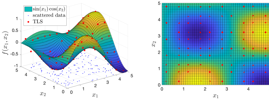
Figure 6.5: TLS reconstructions of f(x_1, x_2) = \sin(x_1)\cos(x_2) on [0,5] \times [0,5] using 25 rectangular elements with randomly distributed data points: side and top view. The TLS reconstruction is evaluated at Gauss-point positions within each element.
