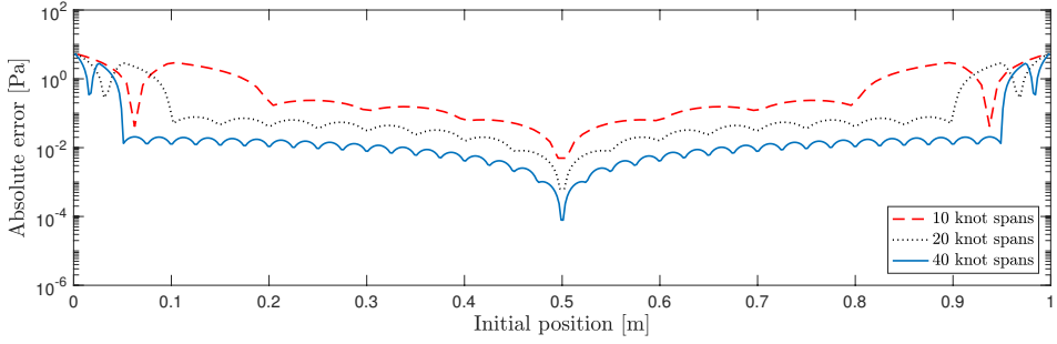
Figure 5.10: Absolute error obtained with BSMPM for stress distribution in the vibrating bar problem without grid crossing.
