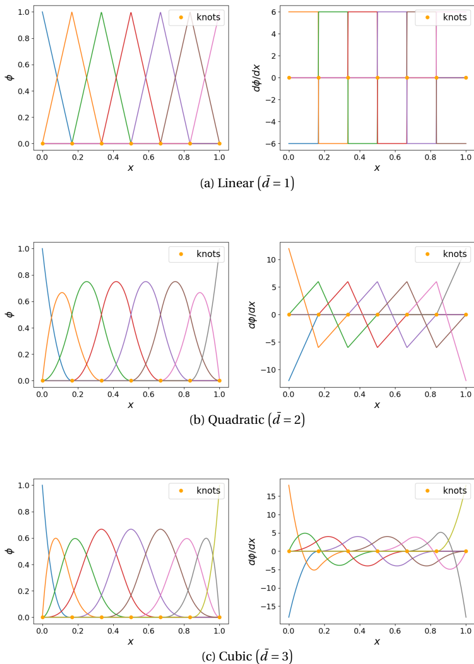
Figure 3.1: Univariate B-spline basis functions and their derivatives.
