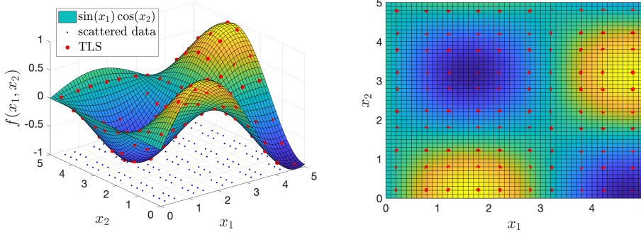
Figure 6.4: TLS reconstructions of f(x_1, x_2) = \sin(x_1)\cos(x_2) on [0,5] \times [0,5] using 25 rectangular elements with 6 data points within each element: side and top view. The TLS reconstruction is evaluated at Gauss-point positions within each element.
