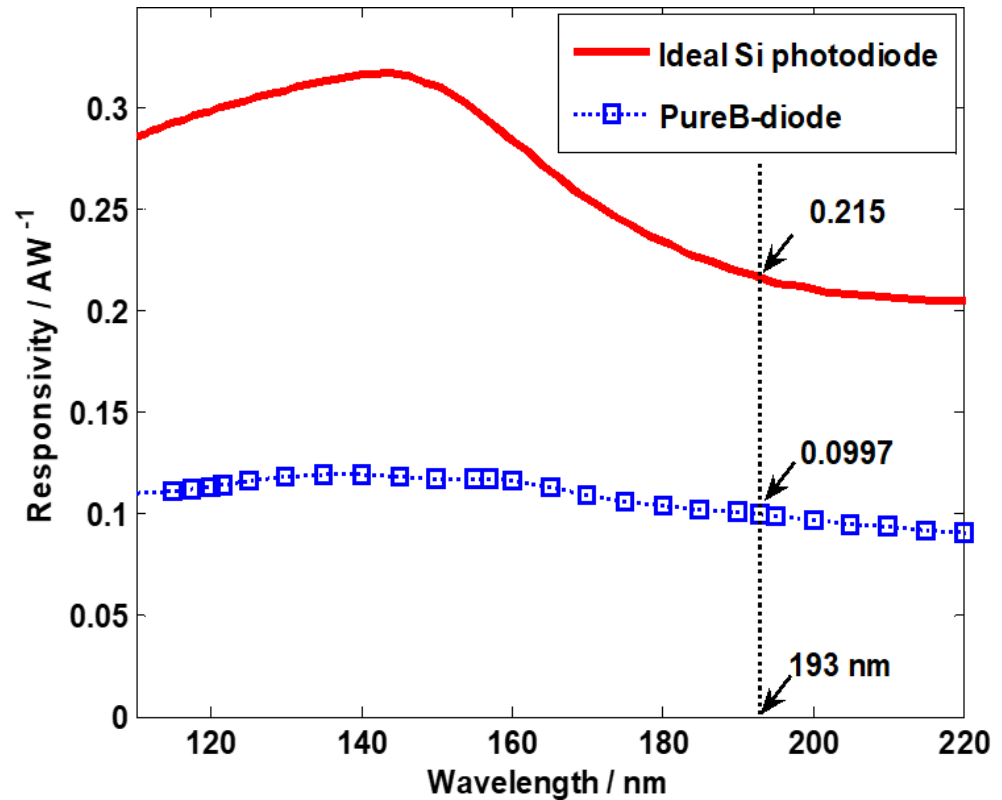
Figure 4. Measured responsivity of a boron-silicon photodiode with \sim 2 nm boron layer, in the deep ultra violet (DUV)/vacuum ultra violet (VUV) spectral ranges, compared with the theoretically attainable values for an ideal Si-based photodetector [19].
