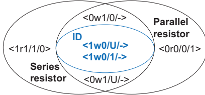
Fig. 11. Static faults.
