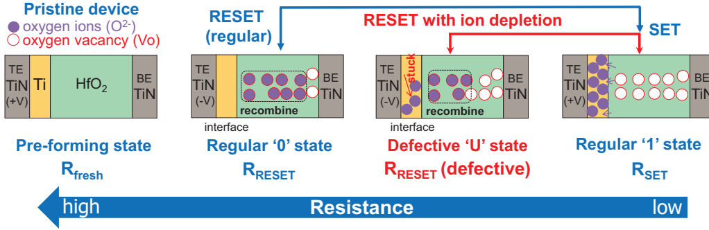
Fig. 5. The schematic view of ion depletion mechanism during RESET process.
