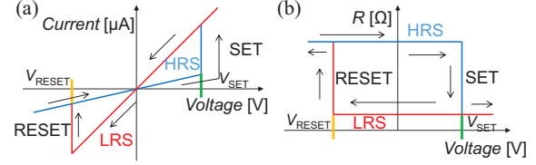
Fig. 2. RRAM electrical switching. (a) Simplified BS switching I-V curve, (b) Simplified BS switching R-V curve.
