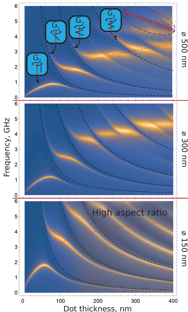
Fig. 2 Simulated thickness ( l ) dependence of the frequencies of the gyrotropic modes for 500 nm, 300 nm, and 150 nm diameter nanodots. Two kinds of approximation curves are used: for a homogenous mode a theoretical dependence 17 of the lowest vortex gyrotropic G_0 frequency is shown as a red dashed line; dashed black curves represent hyperbolae \sim l^{-b} fits of the high frequency and high thickness asymptotes of modes. Colour represents the in-plane microwave magnetic field response intensity of the vortex gyromodes.
