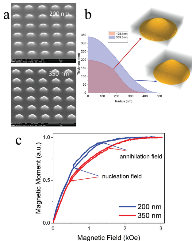
Fig. 4 (a) Scanning electron microscopy images of 200 nm and 350 nm high nanodot arrays; (b) permalloy nanodot profiles derived from atomic force microscopy and renders of the model shapes of averaged nanodots for samples with 200 nm and 350 nm thick nanodots; (c) First quadrant of magnetization hysteretic loops for corresponding nanodot arrays. Nucleation and annihilation fields indicated with arrows.
