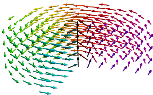
Fig. 1 Cylindrical magnetic dot in the vortex state (not to scale), arrows represent spin momenta directions of individual spins in the cubic lattice. The color of the spins corresponds to the direction of the planar component of the spin, spins on the axis of the particle point out of plane and form the core of the magnetic vortex.
