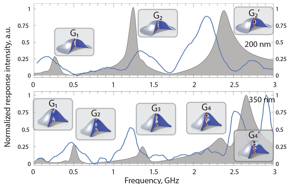
Fig. 5 The microwave absorption spectrum of the 200 nm and 350 nm high nanodot arrays (blue solid lines), and a simulated response of a corresponding idealized infinite arrays composed of the model magnetic nanodots with a period 1\ \mu\text{m} (filled solid black line). Peaks are annotated with renders of corresponding simulated resonant mode intensity cross-sections. Modes are named using a scheme counting the number of the gyrational standing wave nodes (alternatively layers in which the vortex core is almost stationary).
