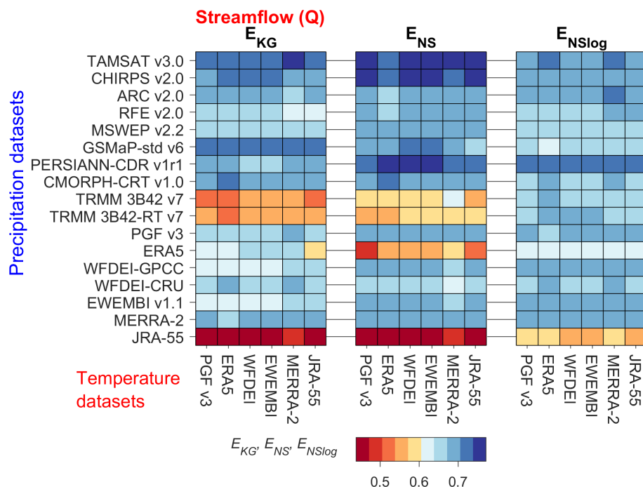
Figure 3. Kling–Gupta efficiency ( E_{KG} ), Nash–Sutcliffe efficiency ( E_{NS} ) and Nash–Sutcliffe efficiency of the logarithm ( E_{NSlog} ) of daily streamflow ( Q ) over the simulation period (2003–2012) for 102 combinations of 17 rainfall datasets (y axis) and 6 temperature datasets (x axis) used as forcing for the hydrological model.
