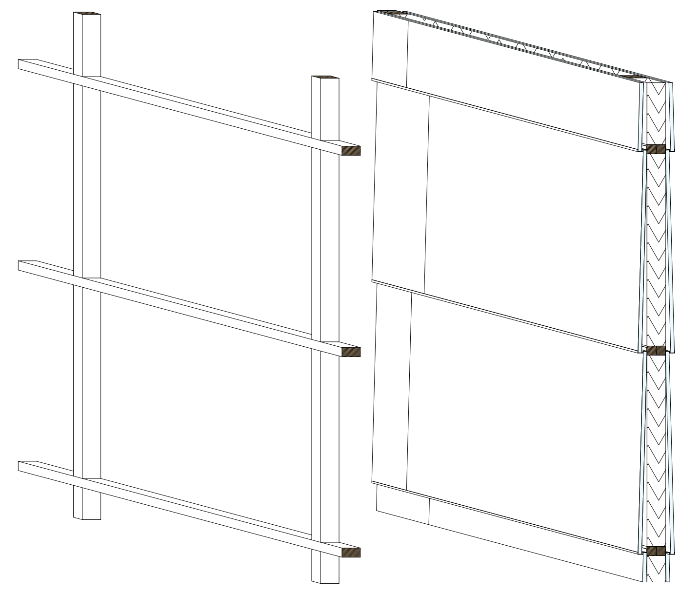
1:20 Build-up inner walls
