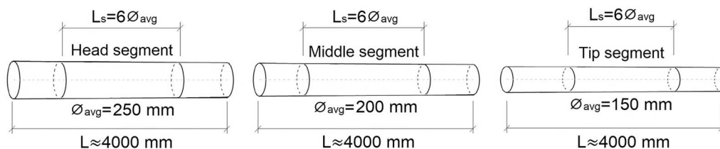
Figure 6. Cutting scheme and subdivision of the full-scale pile into head, middle and tip segments.
