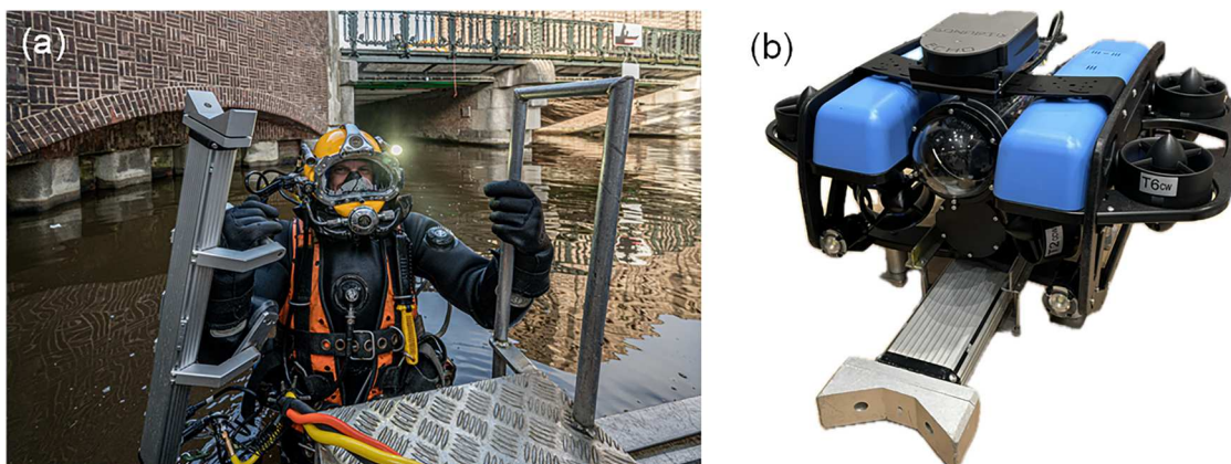
Figure 12. Micro-drilling conducted underwater on wooden piles by: (a) diver, and (b) prototype of ROV incorporating a micro-drilling tool developed by Baars-CIPRO (Baars-CIPRO 2024).
